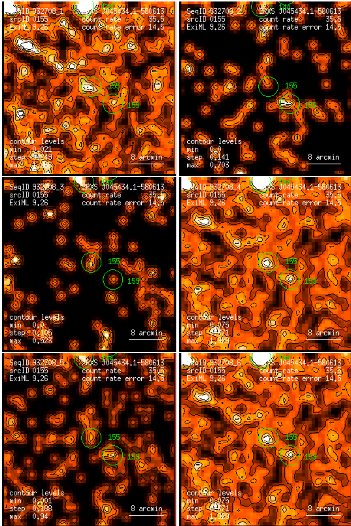
Figure 155: RASS 932708: detection 0155: band rate images, Gaussian filter: (1) PSPC channels 11 – 41, (2) 52 – 90, (3) 91 – 201, (4) 11 – 235, (5) 52 – 201, (6) 11 – 201. Broad band rates in counts/ks. Band rate contour levels in counts/ks/arcmin 2 .
