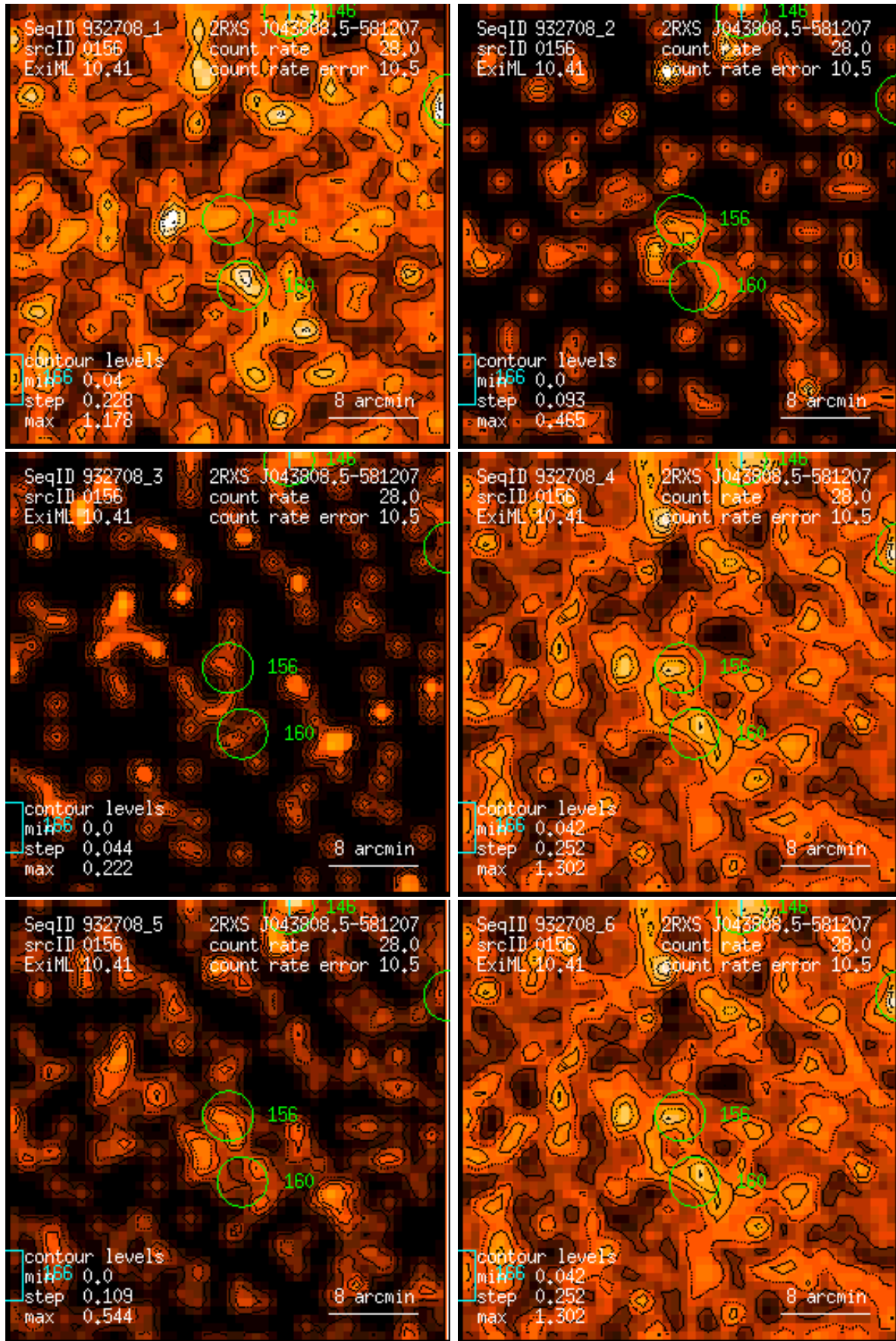
Figure 156: RASS 932708: detection 0156: band rate images, Gaussian filter: (1) PSPC channels 11 – 41, (2) 52 – 90, (3) 91 – 201, (4) 11 – 235, (5) 52 – 201, (6) 11 – 201. Broad band rates in counts/ks. Band rate contour levels in counts/ks/arcmin 2 .
