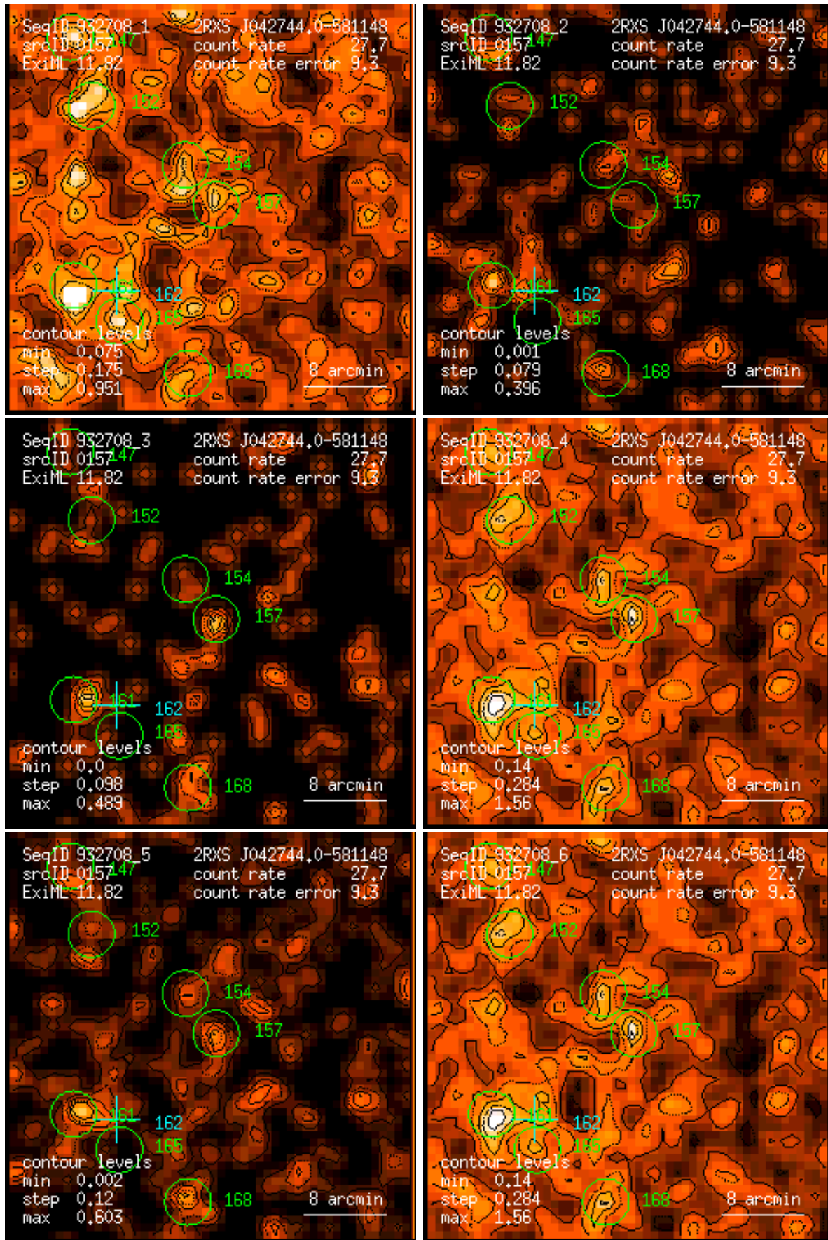
Figure 157: RASS 932708: detection 0157: band rate images, Gaussian filter: (1) PSPC channels 11 – 41, (2) 52 – 90, (3) 91 – 201, (4) 11 – 235, (5) 52 – 201, (6) 11 – 201. Broad band rates in counts/ks. Band rate contour levels in counts/ks/arcmin 2 .
