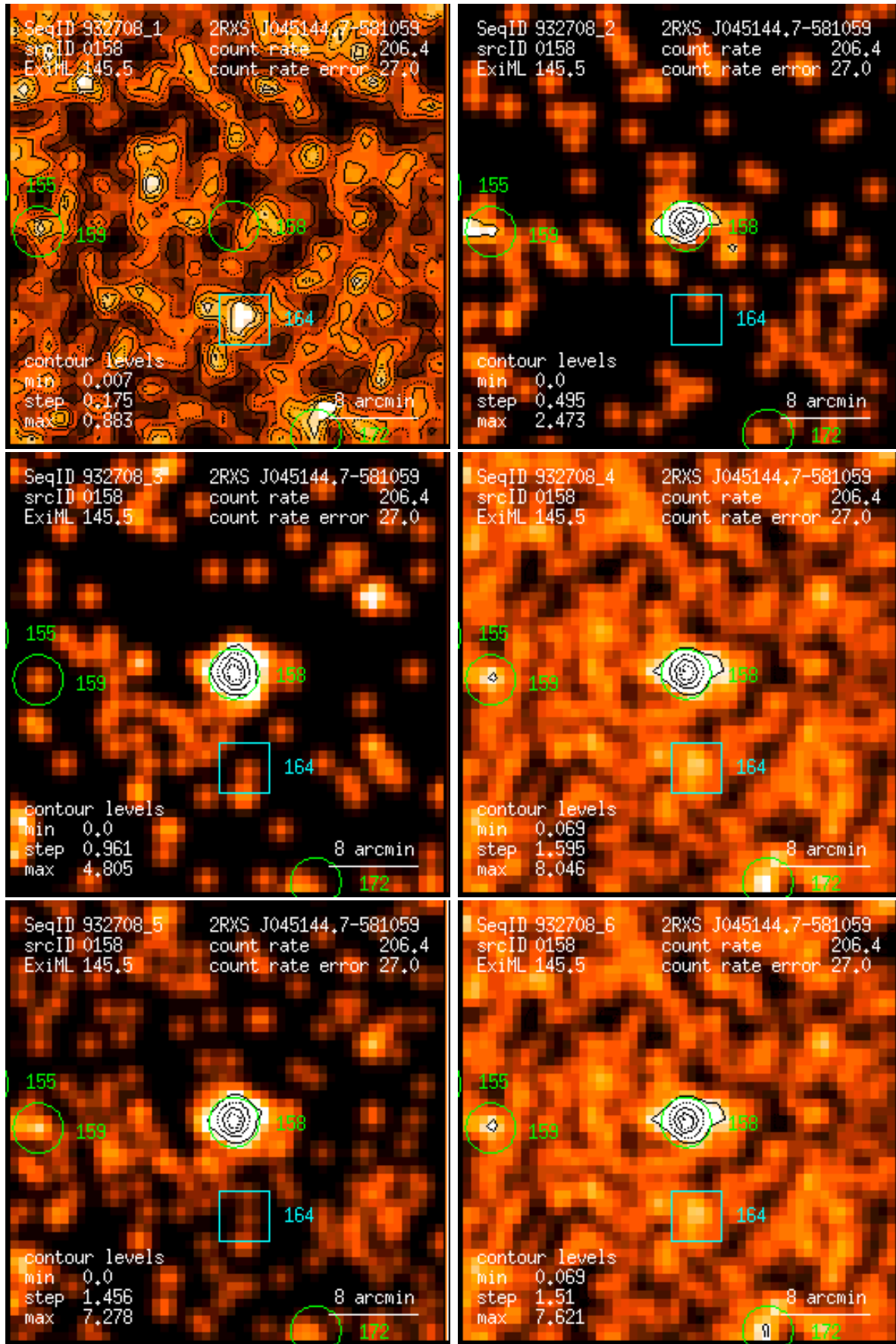
Figure 158: RASS 932708: detection 0158: band rate images, Gaussian filter: (1) PSPC channels 11 – 41, (2) 52 – 90, (3) 91 – 201, (4) 11 – 235, (5) 52 – 201, (6) 11 – 201. Broad band rates in counts/ks. Band rate contour levels in counts/ks/arcmin 2 .
