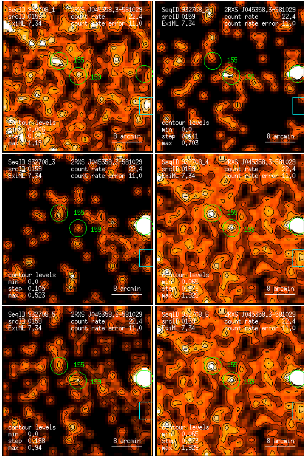
Figure 159: RASS 932708: detection 0159: band rate images, Gaussian filter: (1) PSPC channels 11 – 41, (2) 52 – 90, (3) 91 – 201, (4) 11 – 235, (5) 52 – 201, (6) 11 – 201. Broad band rates in counts/ks. Band rate contour levels in counts/ks/arcmin 2 .
