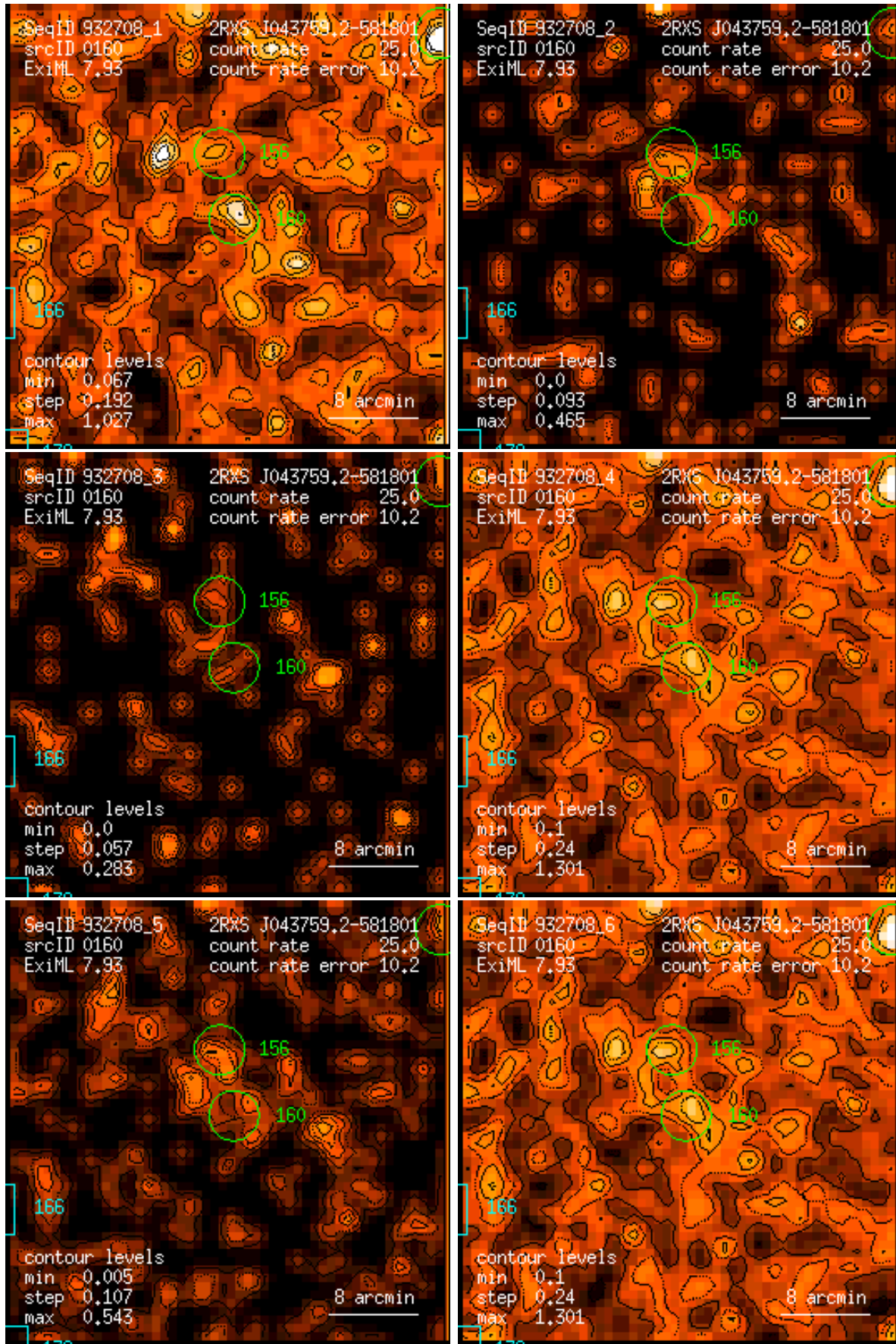
Figure 160: RASS 932708: detection 0160: band rate images, Gaussian filter: (1) PSPC channels 11 – 41, (2) 52 – 90, (3) 91 – 201, (4) 11 – 235, (5) 52 – 201, (6) 11 – 201. Broad band rates in counts/ks. Band rate contour levels in counts/ks/arcmin 2 .
