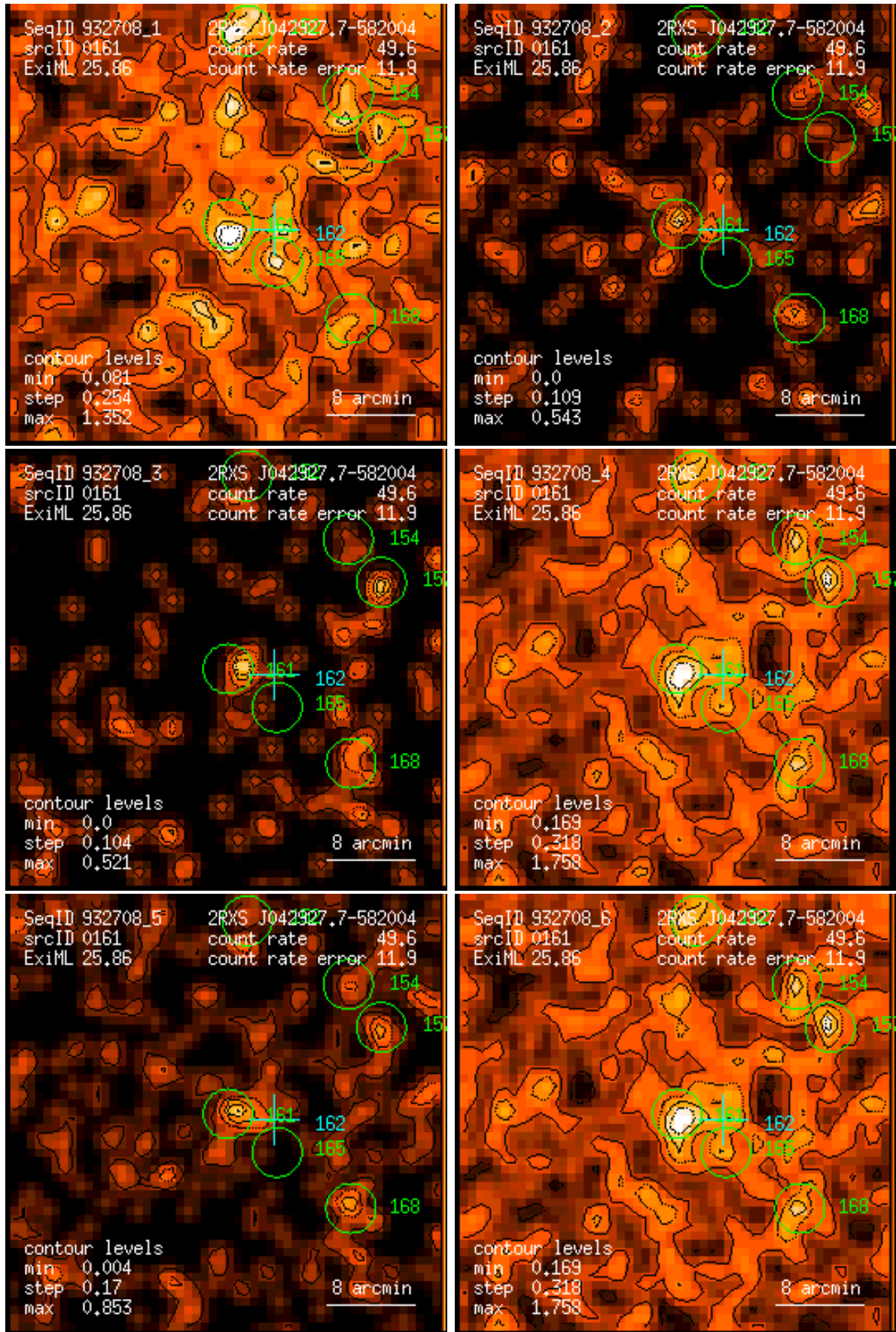
Figure 161: RASS 932708: detection 0161: band rate images, Gaussian filter: (1) PSPC channels 11 – 41, (2) 52 – 90, (3) 91 – 201, (4) 11 – 235, (5) 52 – 201, (6) 11 – 201. Broad band rates in counts/ks. Band rate contour levels in counts/ks/arcmin 2 .
