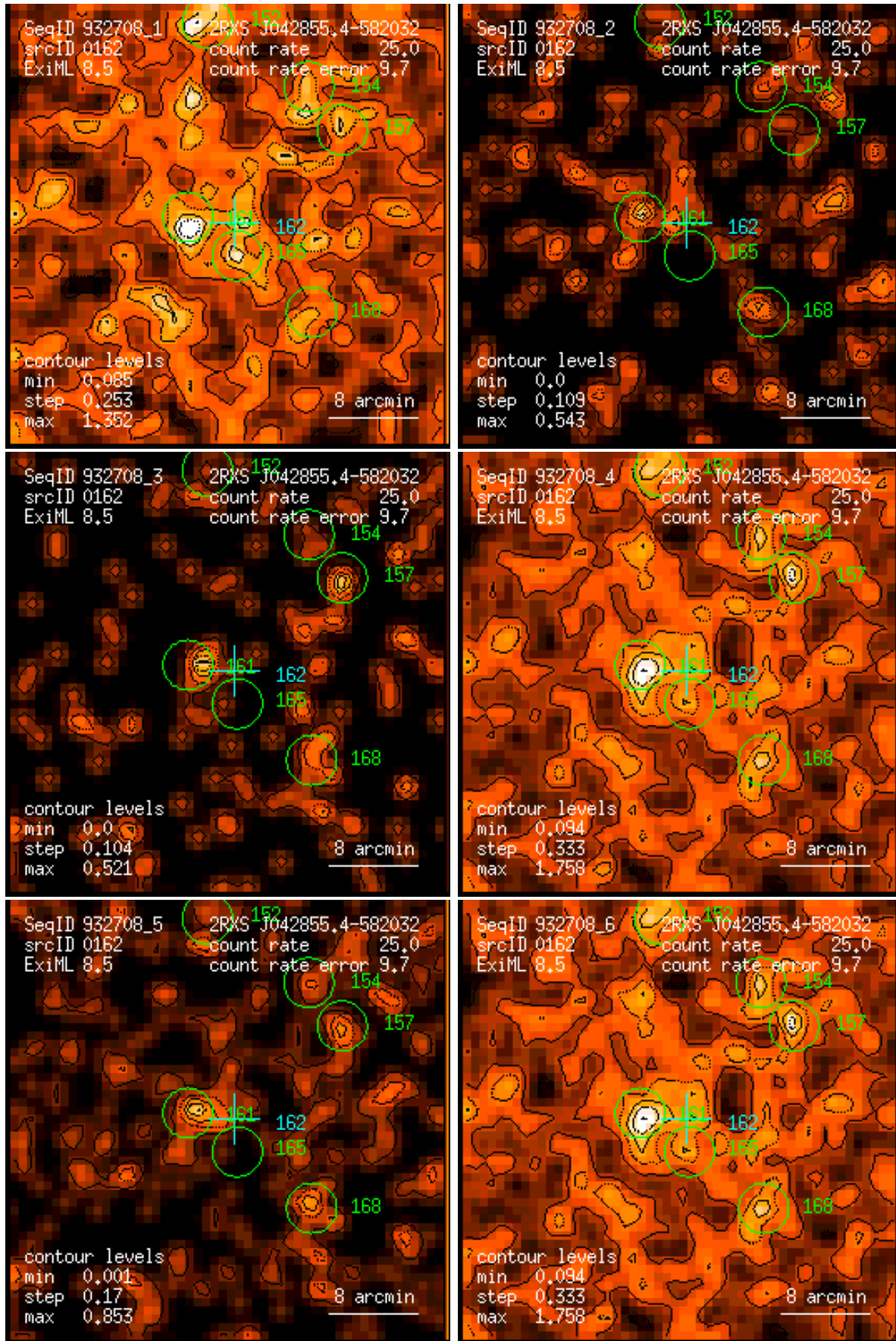
Figure 162: RASS 932708: detection 0162: band rate images, Gaussian filter: (1) PSPC channels 11 – 41, (2) 52 – 90, (3) 91 – 201, (4) 11 – 235, (5) 52 – 201, (6) 11 – 201. Broad band rates in counts/ks. Band rate contour levels in counts/ks/arcmin 2 .
