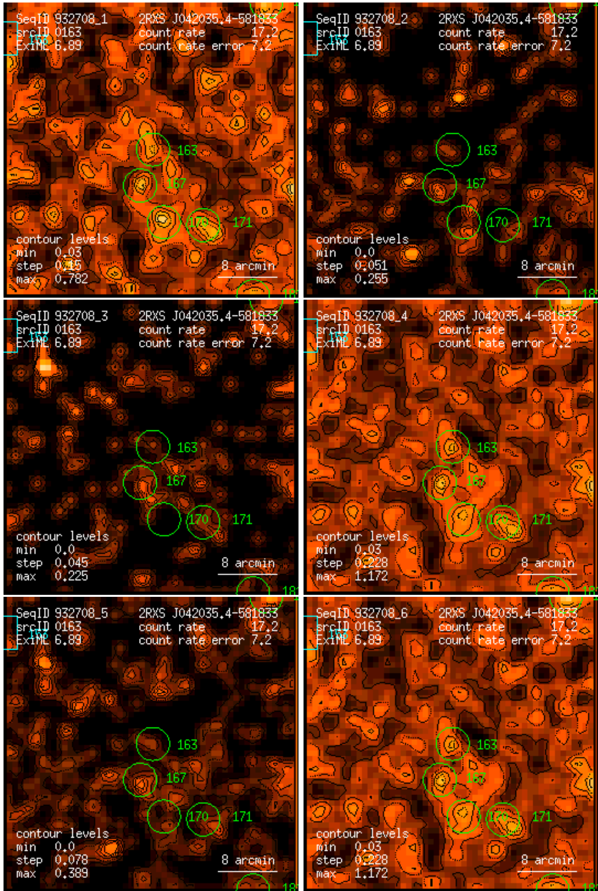
Figure 163: RASS 932708: detection 0163: band rate images, Gaussian filter: (1) PSPC channels 11 – 41, (2) 52 – 90, (3) 91 – 201, (4) 11 – 235, (5) 52 – 201, (6) 11 – 201. Broad band rates in counts/ks. Band rate contour levels in counts/ks/arcmin 2 .
