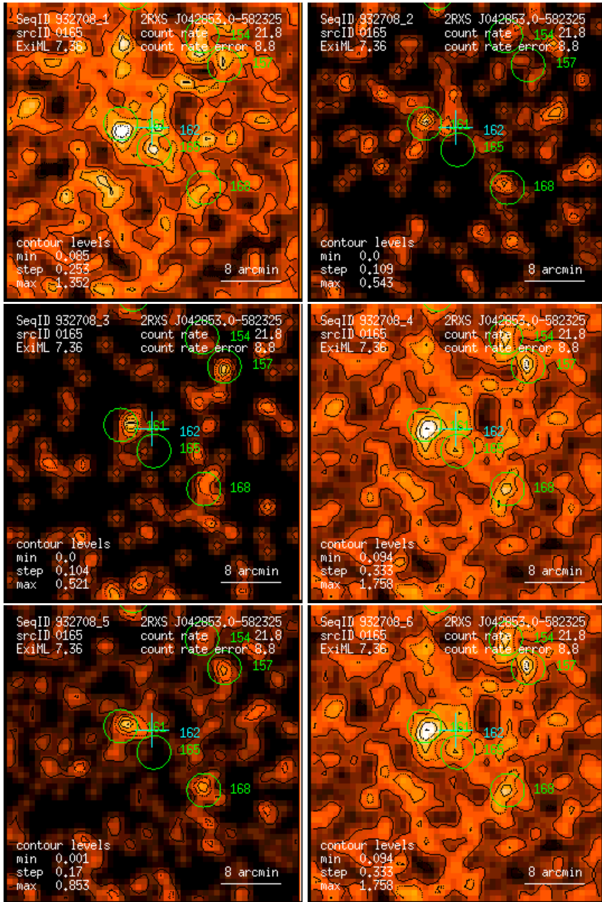
Figure 165: RASS 932708: detection 0165: band rate images, Gaussian filter: (1) PSPC channels 11 – 41, (2) 52 – 90, (3) 91 – 201, (4) 11 – 235, (5) 52 – 201, (6) 11 – 201. Broad band rates in counts/ks. Band rate contour levels in counts/ks/arcmin 2 .
