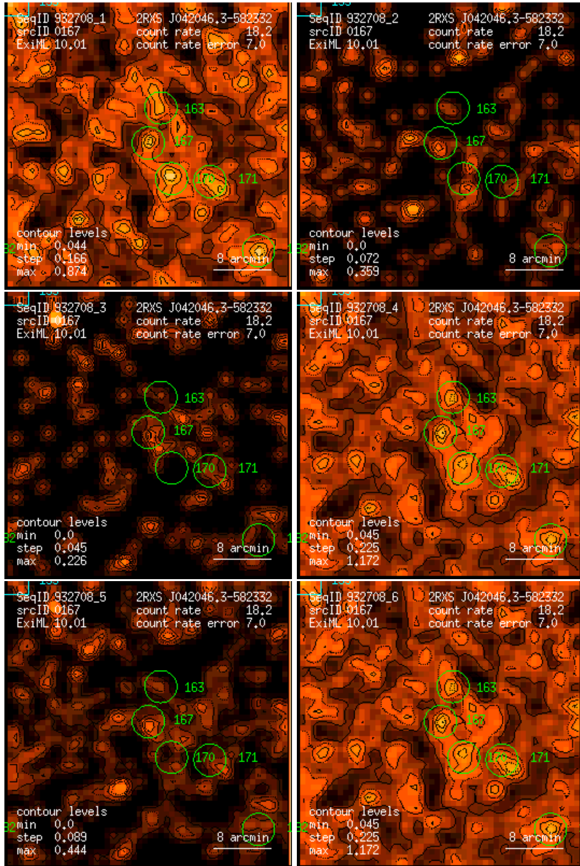
Figure 167: RASS 932708: detection 0167: band rate images, Gaussian filter: (1) PSPC channels 11 – 41, (2) 52 – 90, (3) 91 – 201, (4) 11 – 235, (5) 52 – 201, (6) 11 – 201. Broad band rates in counts/ks. Band rate contour levels in counts/ks/arcmin 2 .
