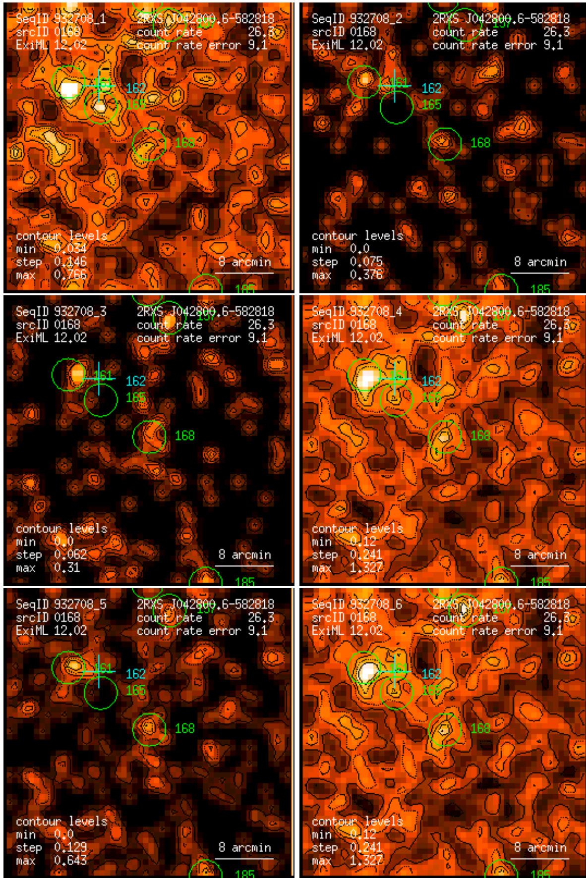
Figure 168: RASS 932708: detection 0168: band rate images, Gaussian filter: (1) PSPC channels 11 – 41, (2) 52 – 90, (3) 91 – 201, (4) 11 – 235, (5) 52 – 201, (6) 11 – 201. Broad band rates in counts/ks. Band rate contour levels in counts/ks/arcmin 2 .
