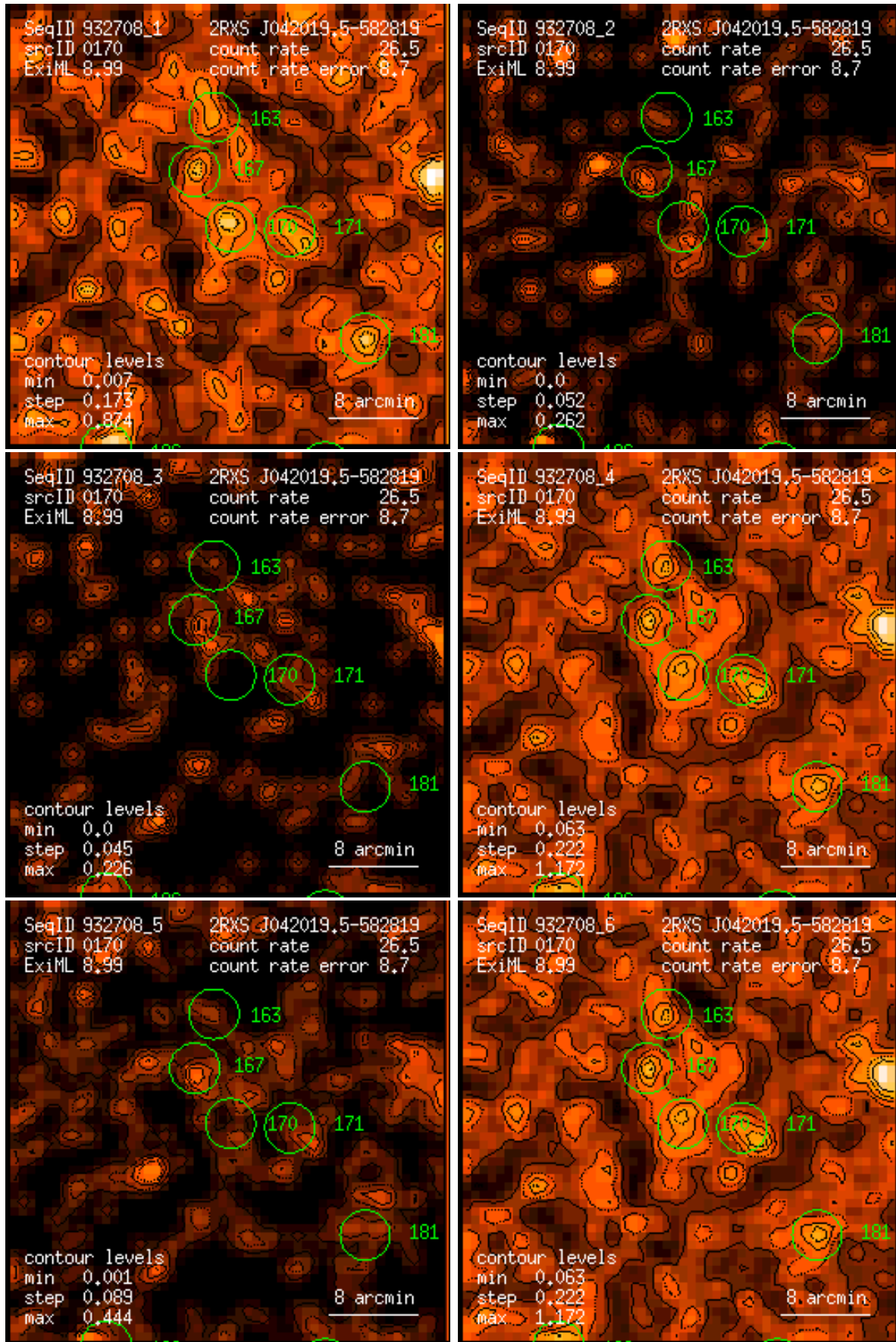
Figure 170: RASS 932708: detection 0170: band rate images, Gaussian filter: (1) PSPC channels 11 – 41, (2) 52 – 90, (3) 91 – 201, (4) 11 – 235, (5) 52 – 201, (6) 11 – 201. Broad band rates in counts/ks. Band rate contour levels in counts/ks/arcmin 2 .
