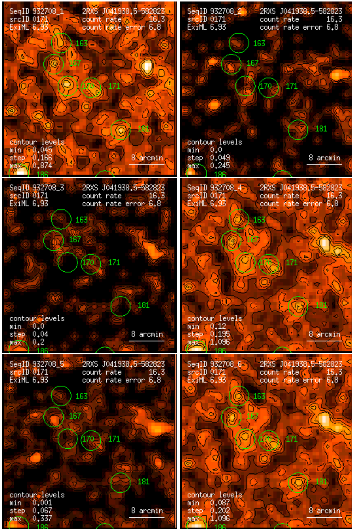
Figure 171: RASS 932708: detection 0171: band rate images, Gaussian filter: (1) PSPC channels 11 – 41, (2) 52 – 90, (3) 91 – 201, (4) 11 – 235, (5) 52 – 201, (6) 11 – 201. Broad band rates in counts/ks. Band rate contour levels in counts/ks/arcmin 2 .
