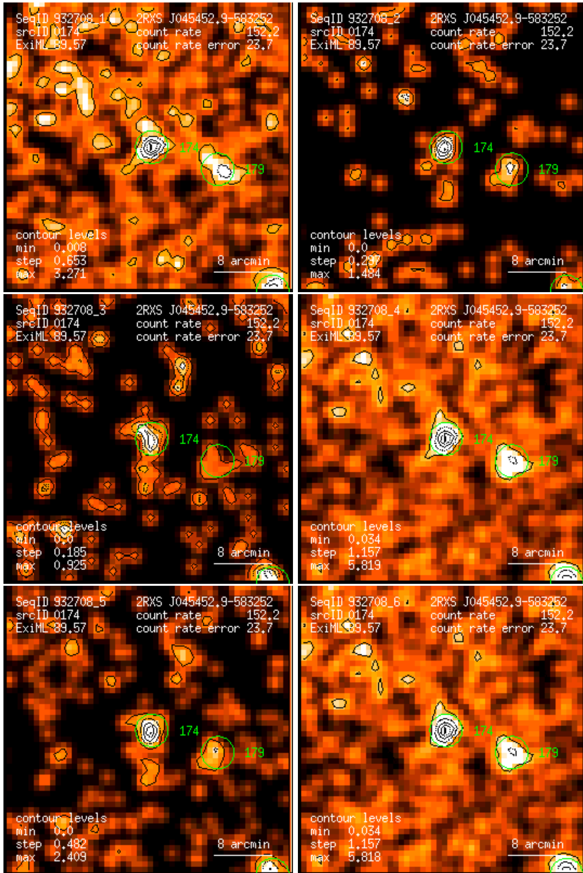
Figure 174: RASS 932708: detection 0174: band rate images, Gaussian filter: (1) PSPC channels 11 – 41, (2) 52 – 90, (3) 91 – 201, (4) 11 – 235, (5) 52 – 201, (6) 11 – 201. Broad band rates in counts/ks. Band rate contour levels in counts/ks/arcmin 2 .
