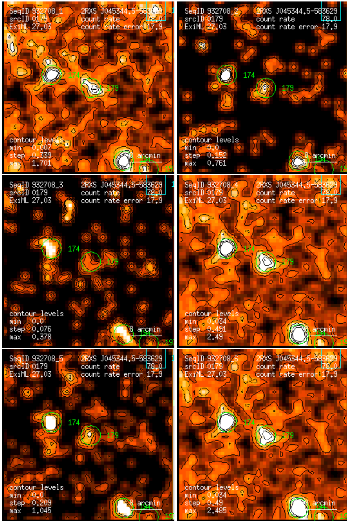
Figure 179: RASS 932708: detection 0179: band rate images, Gaussian filter: (1) PSPC channels 11 – 41, (2) 52 – 90, (3) 91 – 201, (4) 11 – 235, (5) 52 – 201, (6) 11 – 201. Broad band rates in counts/ks. Band rate contour levels in counts/ks/arcmin 2 .
