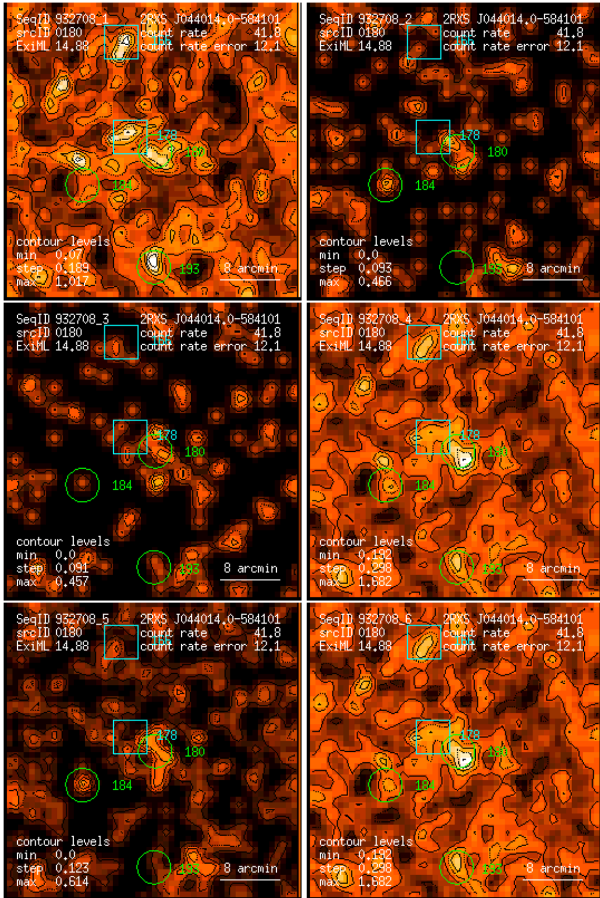
Figure 180: RASS 932708: detection 0180: band rate images, Gaussian filter: (1) PSPC channels 11 – 41, (2) 52 – 90, (3) 91 – 201, (4) 11 – 235, (5) 52 – 201, (6) 11 – 201. Broad band rates in counts/ks. Band rate contour levels in counts/ks/arcmin 2 .
