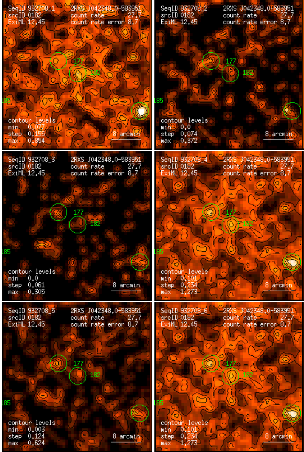
Figure 182: RASS 932708: detection 0182: band rate images, Gaussian filter: (1) PSPC channels 11 – 41, (2) 52 – 90, (3) 91 – 201, (4) 11 – 235, (5) 52 – 201, (6) 11 – 201. Broad band rates in counts/ks. Band rate contour levels in counts/ks/arcmin 2 .
