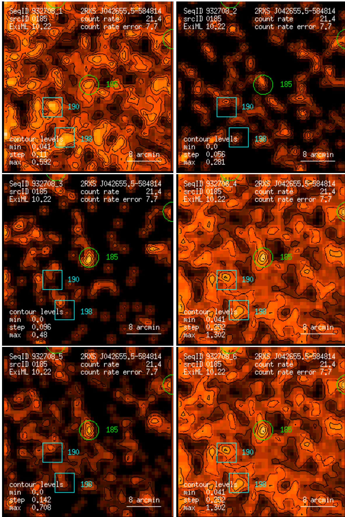
Figure 185: RASS 932708: detection 0185: band rate images, Gaussian filter: (1) PSPC channels 11 – 41, (2) 52 – 90, (3) 91 – 201, (4) 11 – 235, (5) 52 – 201, (6) 11 – 201. Broad band rates in counts/ks. Band rate contour levels in counts/ks/arcmin 2 .
