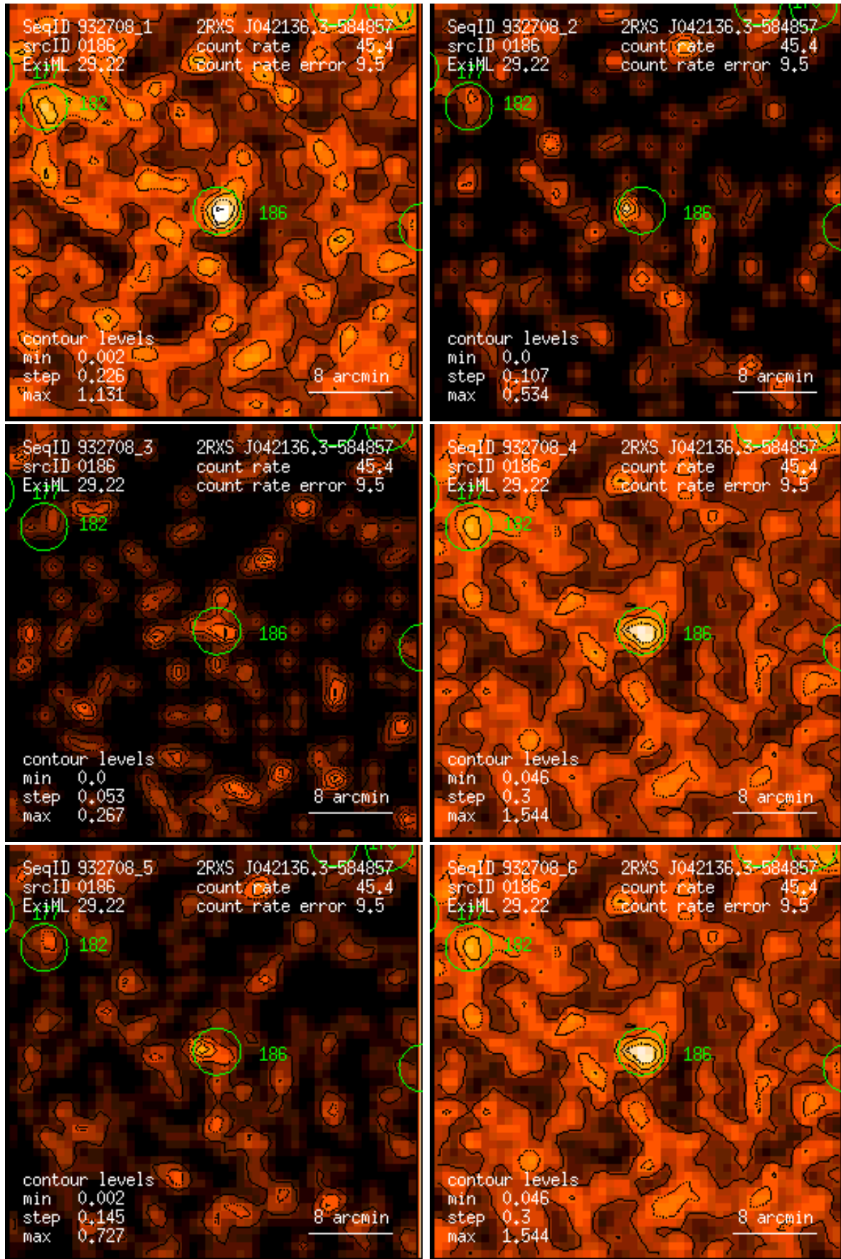
Figure 186: RASS 932708: detection 0186: band rate images, Gaussian filter: (1) PSPC channels 11 – 41, (2) 52 – 90, (3) 91 – 201, (4) 11 – 235, (5) 52 – 201, (6) 11 – 201. Broad band rates in counts/ks. Band rate contour levels in counts/ks/arcmin 2 .
