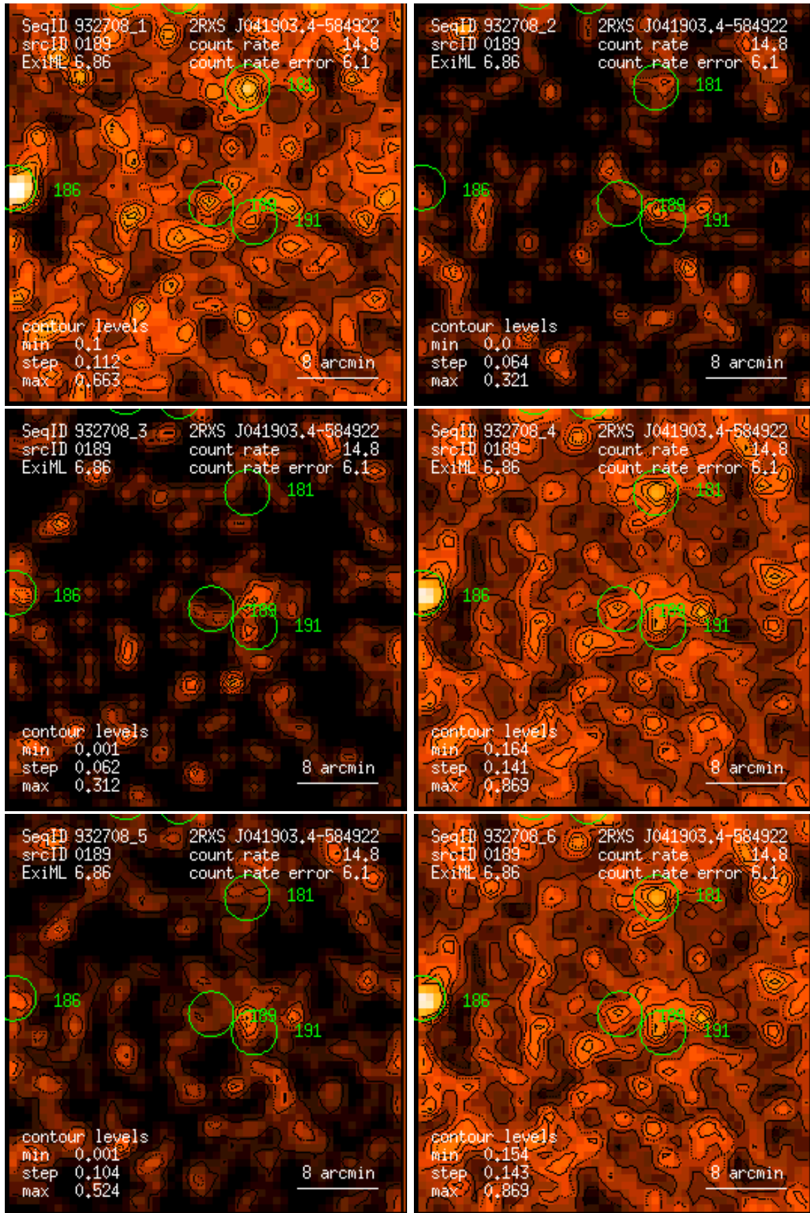
Figure 189: RASS 932708: detection 0189: band rate images, Gaussian filter: (1) PSPC channels 11 – 41, (2) 52 – 90, (3) 91 – 201, (4) 11 – 235, (5) 52 – 201, (6) 11 – 201. Broad band rates in counts/ks. Band rate contour levels in counts/ks/arcmin 2 .
