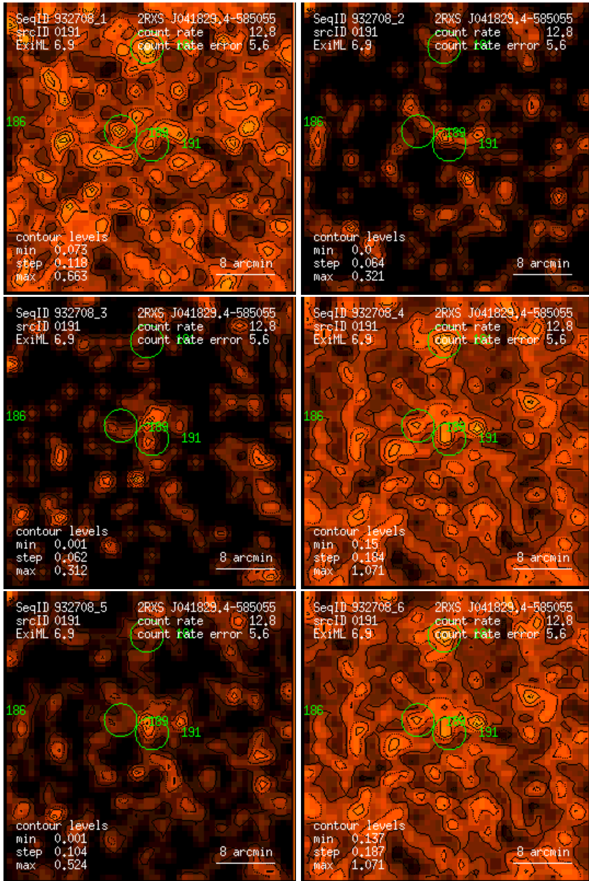
Figure 191: RASS 932708: detection 0191: band rate images, Gaussian filter: (1) PSPC channels 11 – 41, (2) 52 – 90, (3) 91 – 201, (4) 11 – 235, (5) 52 – 201, (6) 11 – 201. Broad band rates in counts/ks. Band rate contour levels in counts/ks/arcmin 2 .
