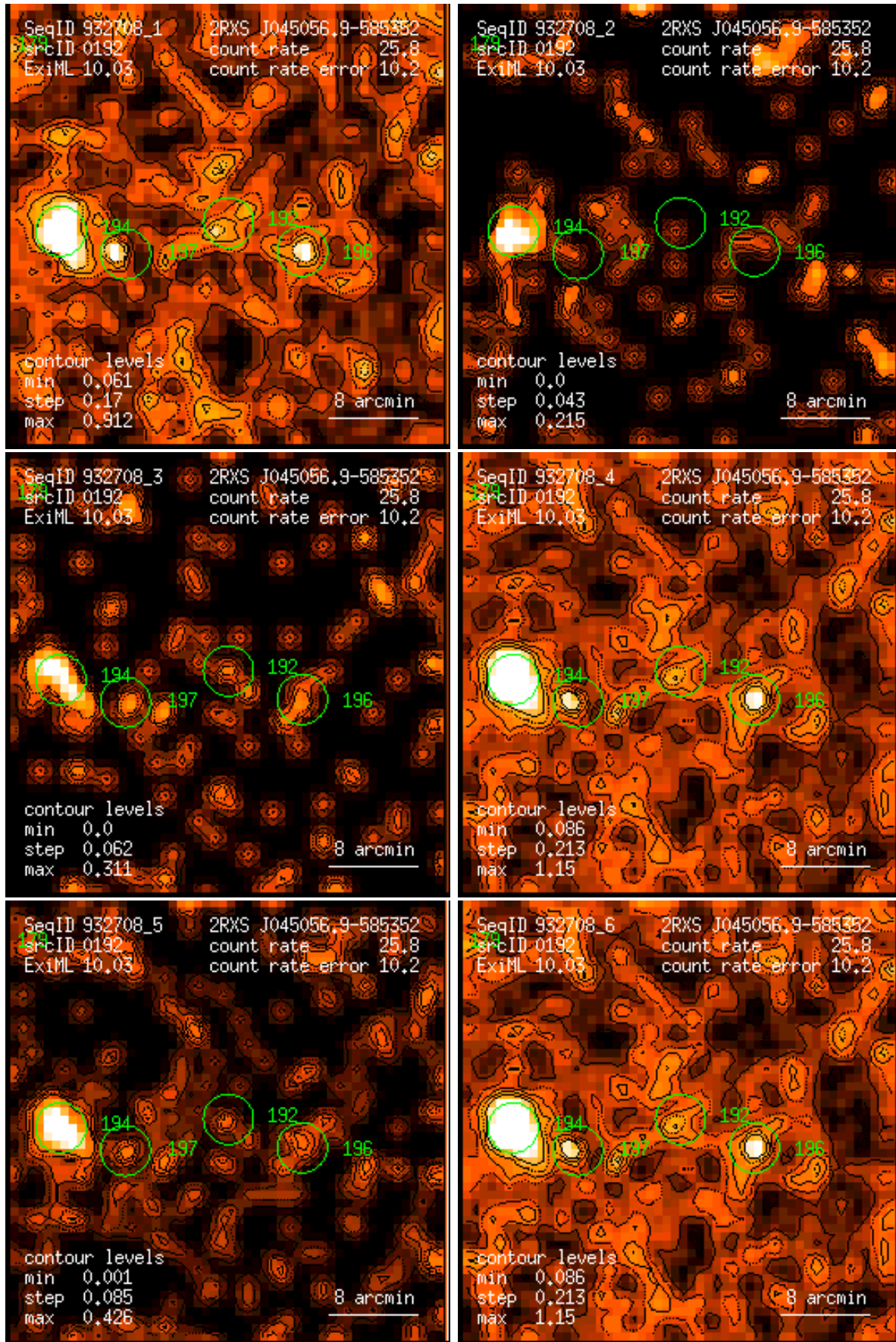
Figure 192: RASS 932708: detection 0192: band rate images, Gaussian filter: (1) PSPC channels 11 – 41, (2) 52 – 90, (3) 91 – 201, (4) 11 – 235, (5) 52 – 201, (6) 11 – 201. Broad band rates in counts/ks. Band rate contour levels in counts/ks/arcmin 2 .
