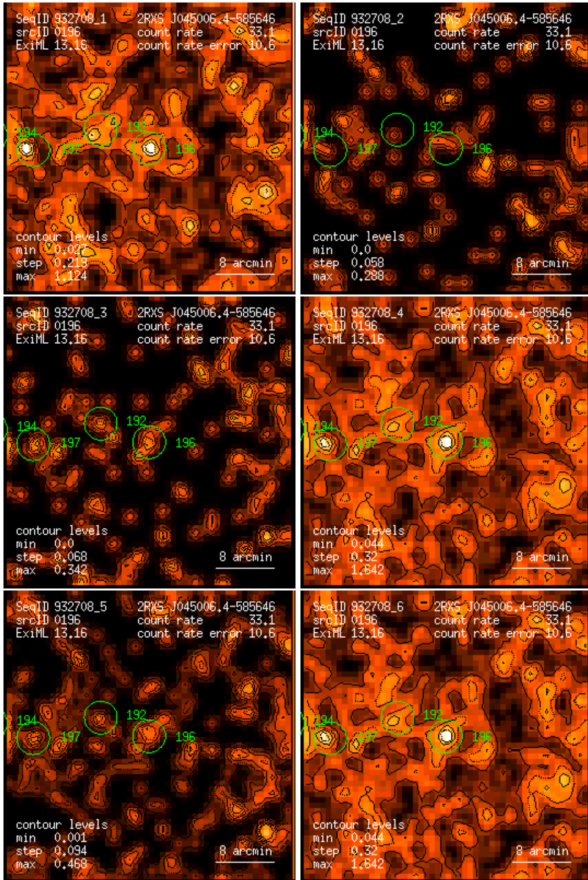
Figure 196: RASS 932708: detection 0196: band rate images, Gaussian filter: (1) PSPC channels 11 – 41, (2) 52 – 90, (3) 91 – 201, (4) 11 – 235, (5) 52 – 201, (6) 11 – 201. Broad band rates in counts/ks. Band rate contour levels in counts/ks/arcmin 2 .
