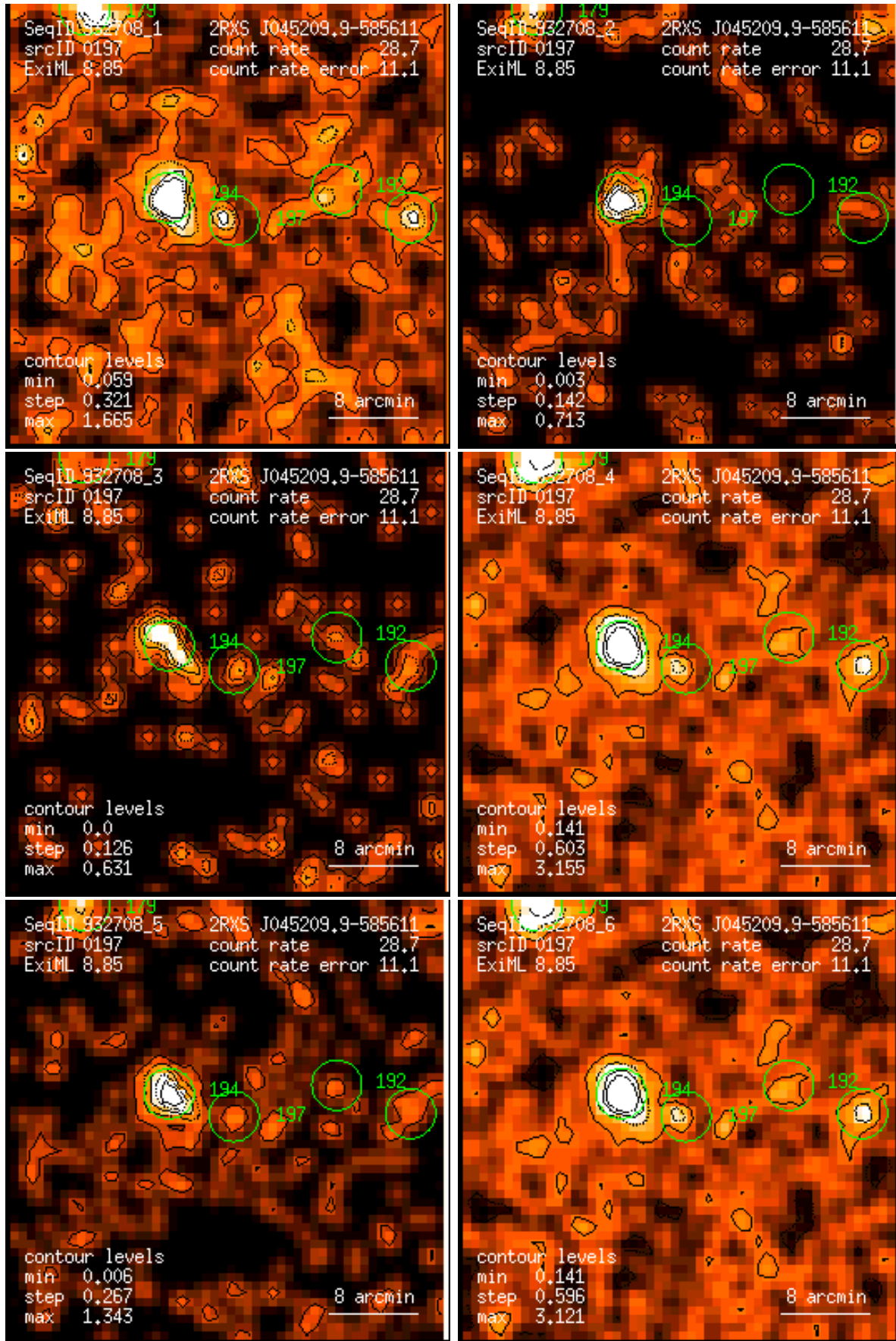
Figure 197: RASS 932708: detection 0197: band rate images, Gaussian filter: (1) PSPC channels 11 – 41, (2) 52 – 90, (3) 91 – 201, (4) 11 – 235, (5) 52 – 201, (6) 11 – 201. Broad band rates in counts/ks. Band rate contour levels in counts/ks/arcmin 2 .
