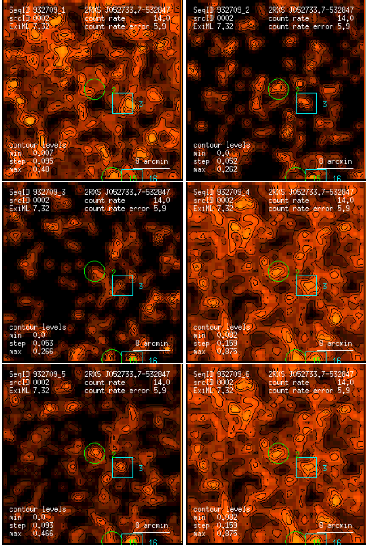
Figure 2: RASS 932709: detection 0002: band rate images, Gaussian filter: (1) PSPC channels 11 – 41, (2) 52 – 90, (3) 91 – 201, (4) 11 – 235, (5) 52 – 201, (6) 11 – 201. Broad band rates in counts/ks. Band rate contour levels in counts/ks/arcmin 2 .
