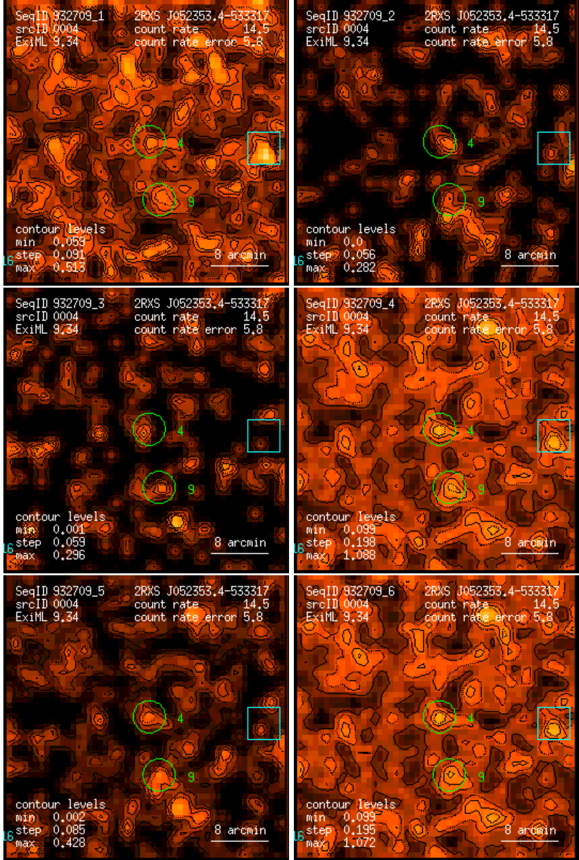
Figure 4: RASS 932709: detection 0004: band rate images, Gaussian filter: (1) PSPC channels 11 – 41, (2) 52 – 90, (3) 91 – 201, (4) 11 – 235, (5) 52 – 201, (6) 11 – 201. Broad band rates in counts/ks. Band rate contour levels in counts/ks/arcmin 2 .
