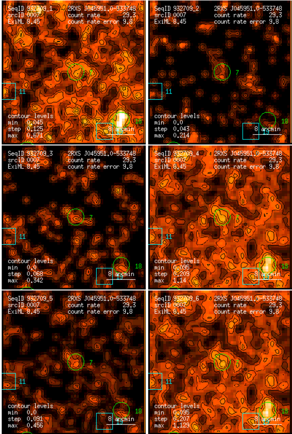
Figure 7: RASS 932709: detection 0007: band rate images, Gaussian filter: (1) PSPC channels 11 – 41, (2) 52 – 90, (3) 91 – 201, (4) 11 – 235, (5) 52 – 201, (6) 11 – 201. Broad band rates in counts/ks. Band rate contour levels in counts/ks/arcmin 2 .
