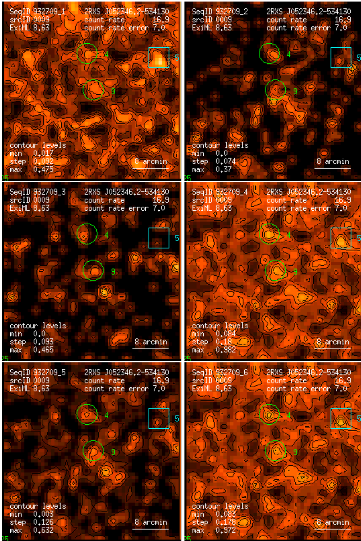
Figure 9: RASS 932709: detection 0009: band rate images, Gaussian filter: (1) PSPC channels 11 – 41, (2) 52 – 90, (3) 91 – 201, (4) 11 – 235, (5) 52 – 201, (6) 11 – 201. Broad band rates in counts/ks. Band rate contour levels in counts/ks/arcmin 2 .
