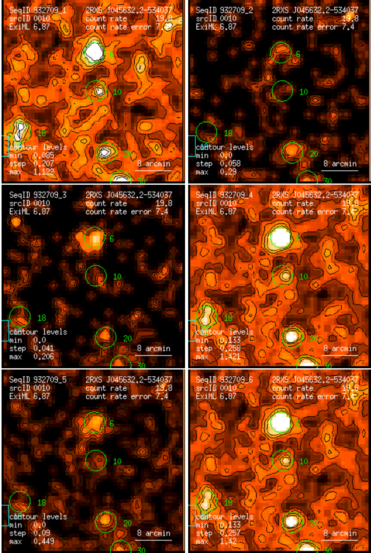
Figure 10: RASS 932709: detection 0010: band rate images, Gaussian filter: (1) PSPC channels 11 – 41, (2) 52 – 90, (3) 91 – 201, (4) 11 – 235, (5) 52 – 201, (6) 11 – 201. Broad band rates in counts/ks. Band rate contour levels in counts/ks/arcmin 2 .
