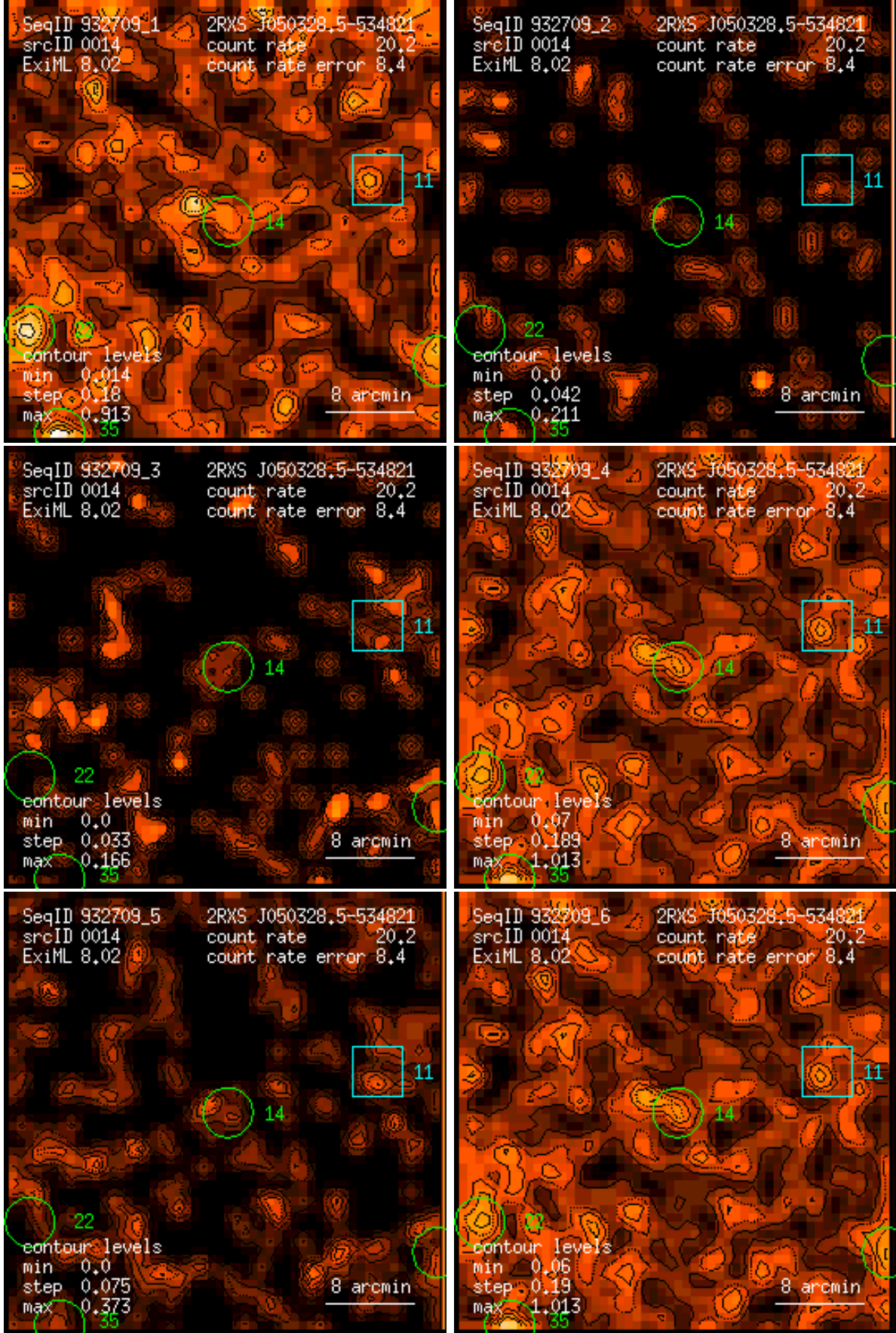
Figure 14: RASS 932709: detection 0014: band rate images, Gaussian filter: (1) PSPC channels 11 – 41, (2) 52 – 90, (3) 91 – 201, (4) 11 – 235, (5) 52 – 201, (6) 11 – 201. Broad band rates in counts/ks. Band rate contour levels in counts/ks/arcmin 2 .
