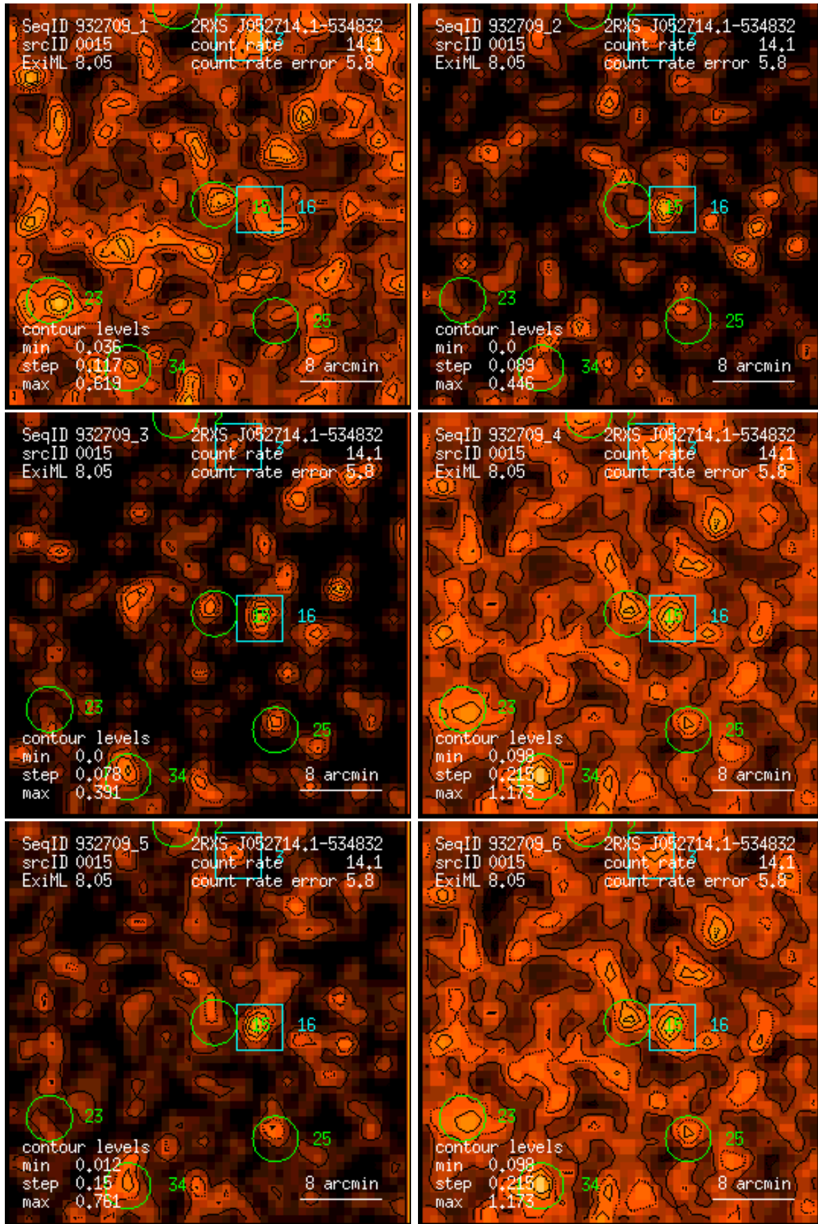
Figure 15: RASS 932709: detection 0015: band rate images, Gaussian filter: (1) PSPC channels 11 – 41, (2) 52 – 90, (3) 91 – 201, (4) 11 – 235, (5) 52 – 201, (6) 11 – 201. Broad band rates in counts/ks. Band rate contour levels in counts/ks/arcmin 2 .
