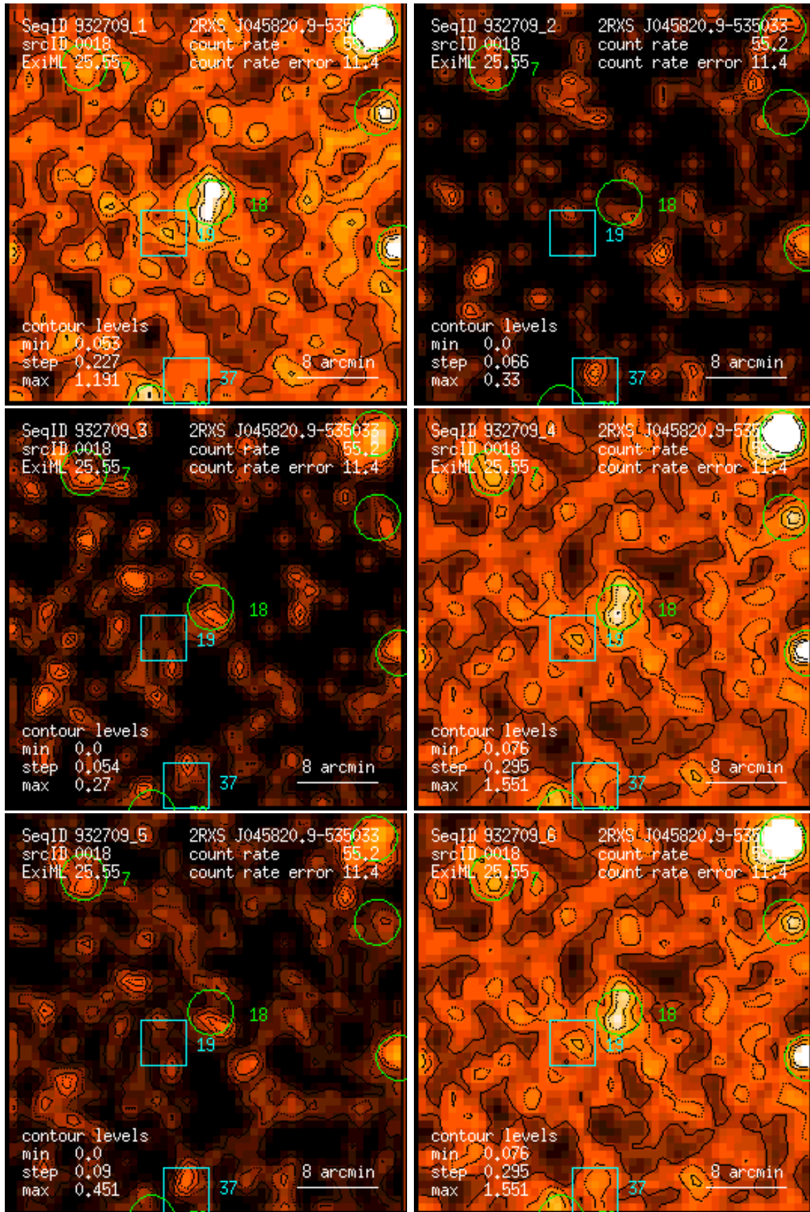
Figure 18: RASS 932709: detection 0018: band rate images, Gaussian filter: (1) PSPC channels 11 – 41, (2) 52 – 90, (3) 91 – 201, (4) 11 – 235, (5) 52 – 201, (6) 11 – 201. Broad band rates in counts/ks. Band rate contour levels in counts/ks/arcmin 2 .
