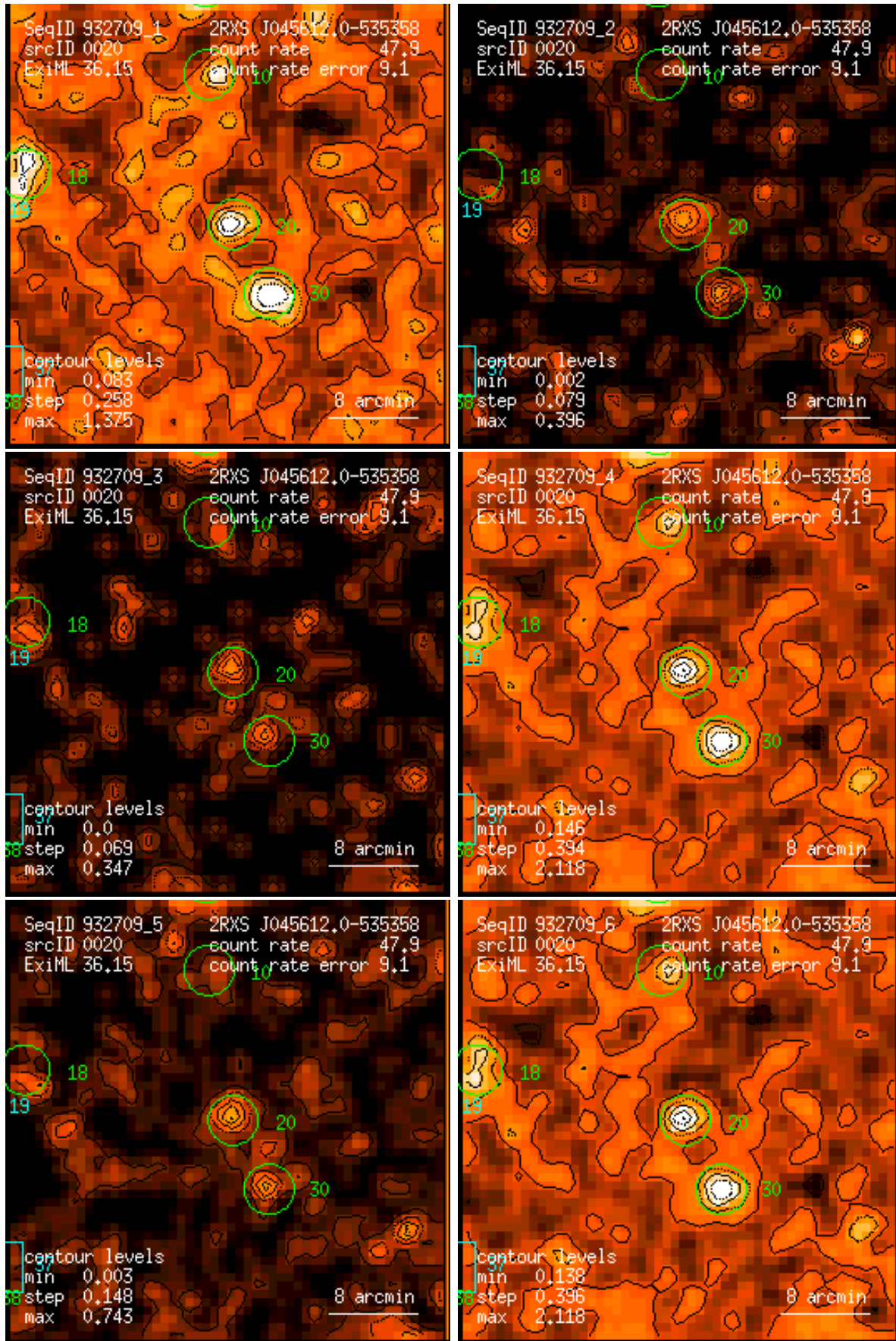
Figure 20: RASS 932709: detection 0020: band rate images, Gaussian filter: (1) PSPC channels 11 – 41, (2) 52 – 90, (3) 91 – 201, (4) 11 – 235, (5) 52 – 201, (6) 11 – 201. Broad band rates in counts/ks. Band rate contour levels in counts/ks/arcmin 2 .
