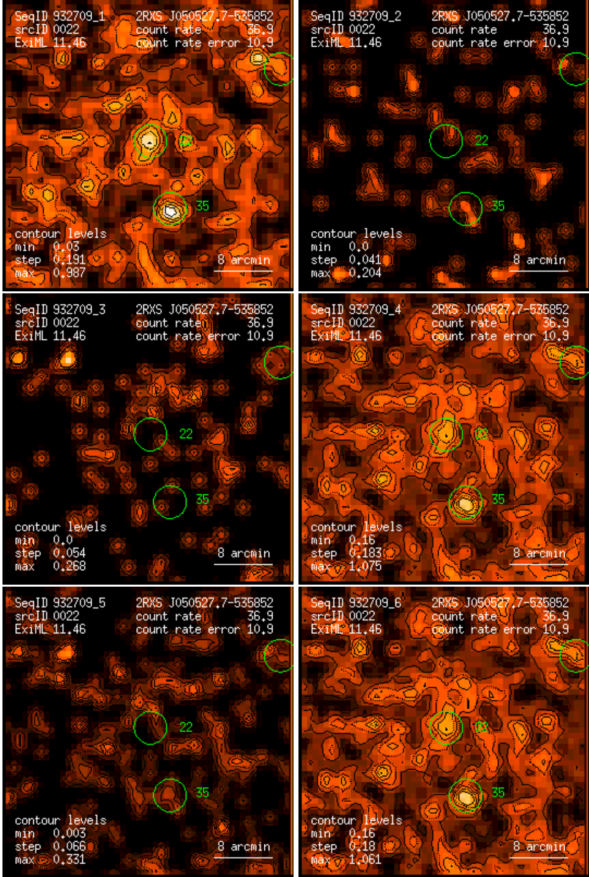
Figure 22: RASS 932709: detection 0022: band rate images, Gaussian filter: (1) PSPC channels 11 – 41, (2) 52 – 90, (3) 91 – 201, (4) 11 – 235, (5) 52 – 201, (6) 11 – 201. Broad band rates in counts/ks. Band rate contour levels in counts/ks/arcmin 2 .
