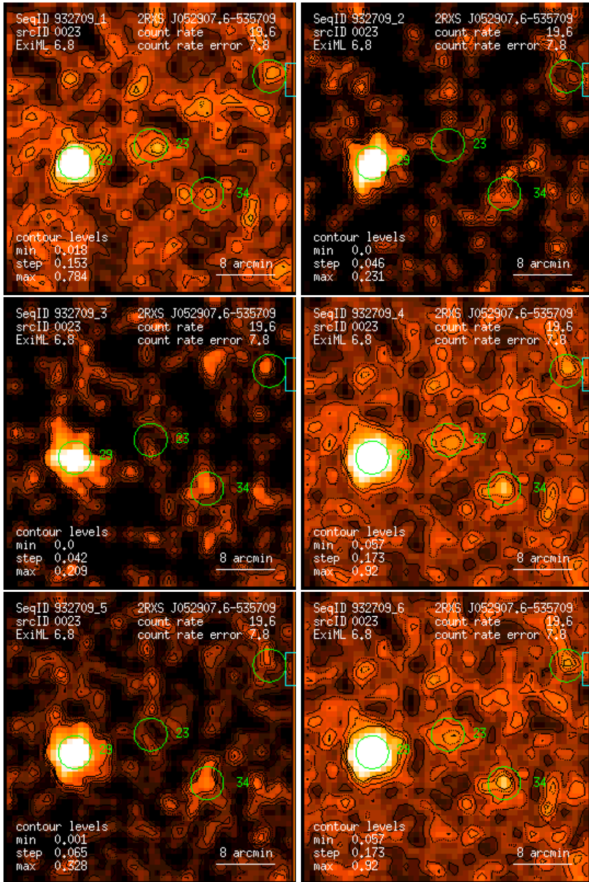
Figure 23: RASS 932709: detection 0023: band rate images, Gaussian filter: (1) PSPC channels 11 – 41, (2) 52 – 90, (3) 91 – 201, (4) 11 – 235, (5) 52 – 201, (6) 11 – 201. Broad band rates in counts/ks. Band rate contour levels in counts/ks/arcmin 2 .
