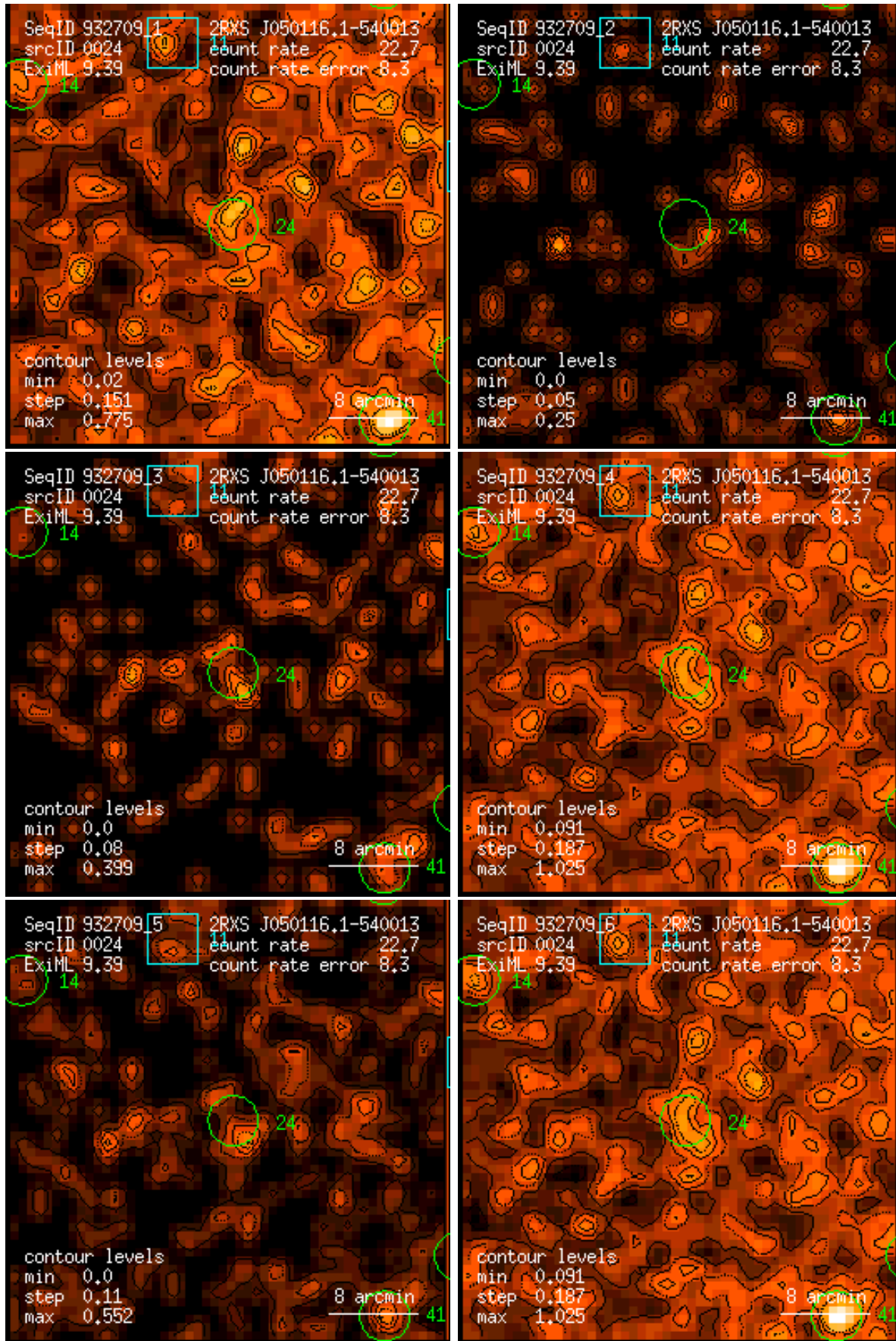
Figure 24: RASS 932709: detection 0024: band rate images, Gaussian filter: (1) PSPC channels 11 – 41, (2) 52 – 90, (3) 91 – 201, (4) 11 – 235, (5) 52 – 201, (6) 11 – 201. Broad band rates in counts/ks. Band rate contour levels in counts/ks/arcmin 2 .
