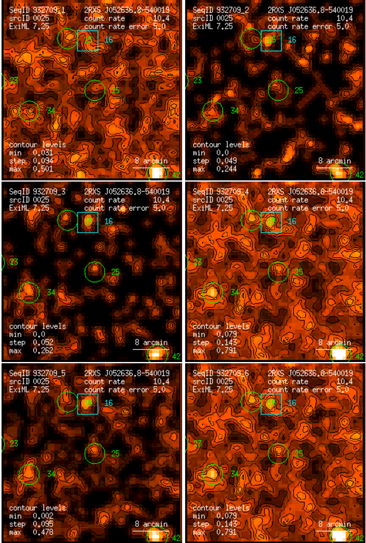
Figure 25: RASS 932709: detection 0025: band rate images, Gaussian filter: (1) PSPC channels 11 – 41, (2) 52 – 90, (3) 91 – 201, (4) 11 – 235, (5) 52 – 201, (6) 11 – 201. Broad band rates in counts/ks. Band rate contour levels in counts/ks/arcmin 2 .
