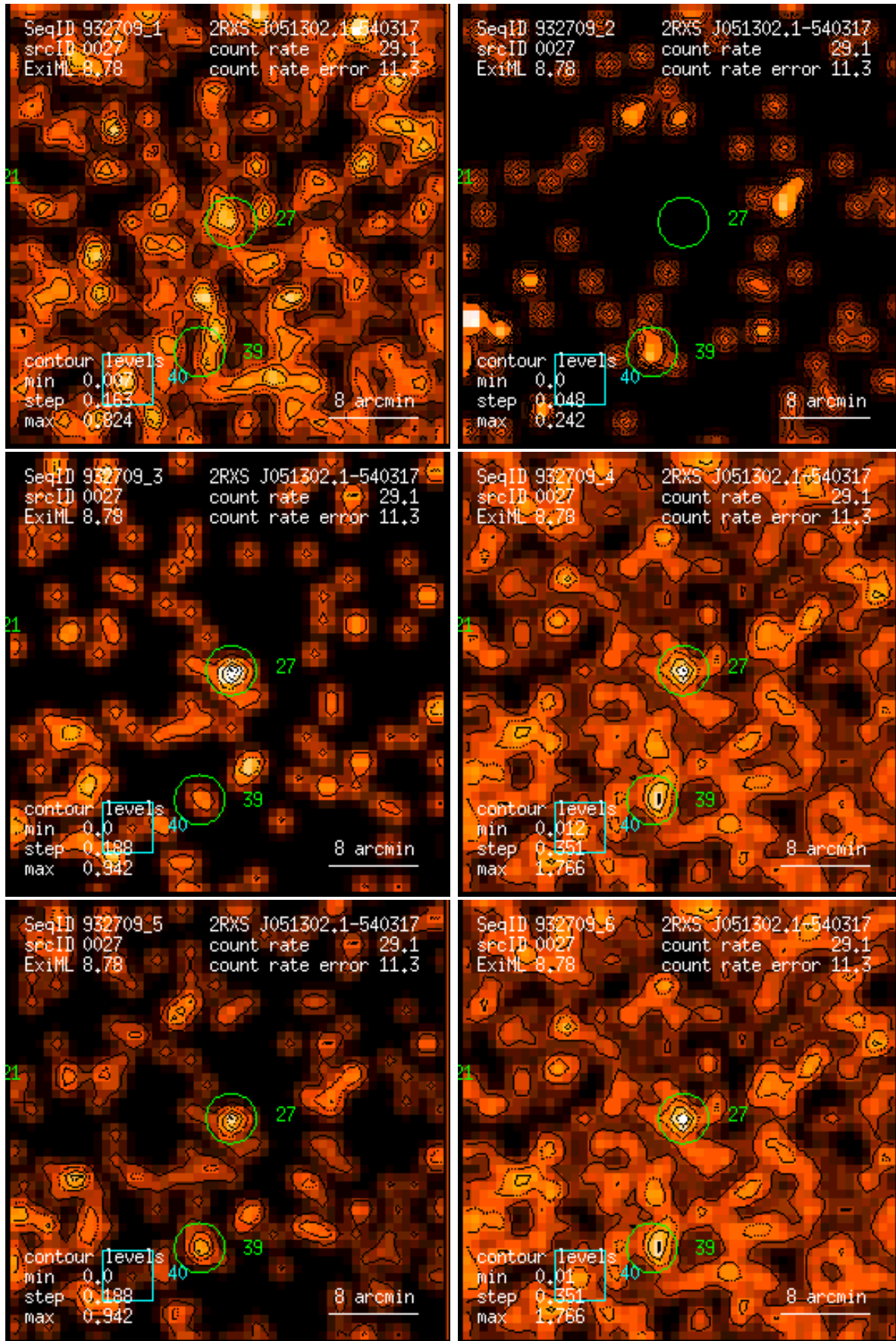
Figure 27: RASS 932709: detection 0027: band rate images, Gaussian filter: (1) PSPC channels 11 – 41, (2) 52 – 90, (3) 91 – 201, (4) 11 – 235, (5) 52 – 201, (6) 11 – 201. Broad band rates in counts/ks. Band rate contour levels in counts/ks/arcmin 2 .
