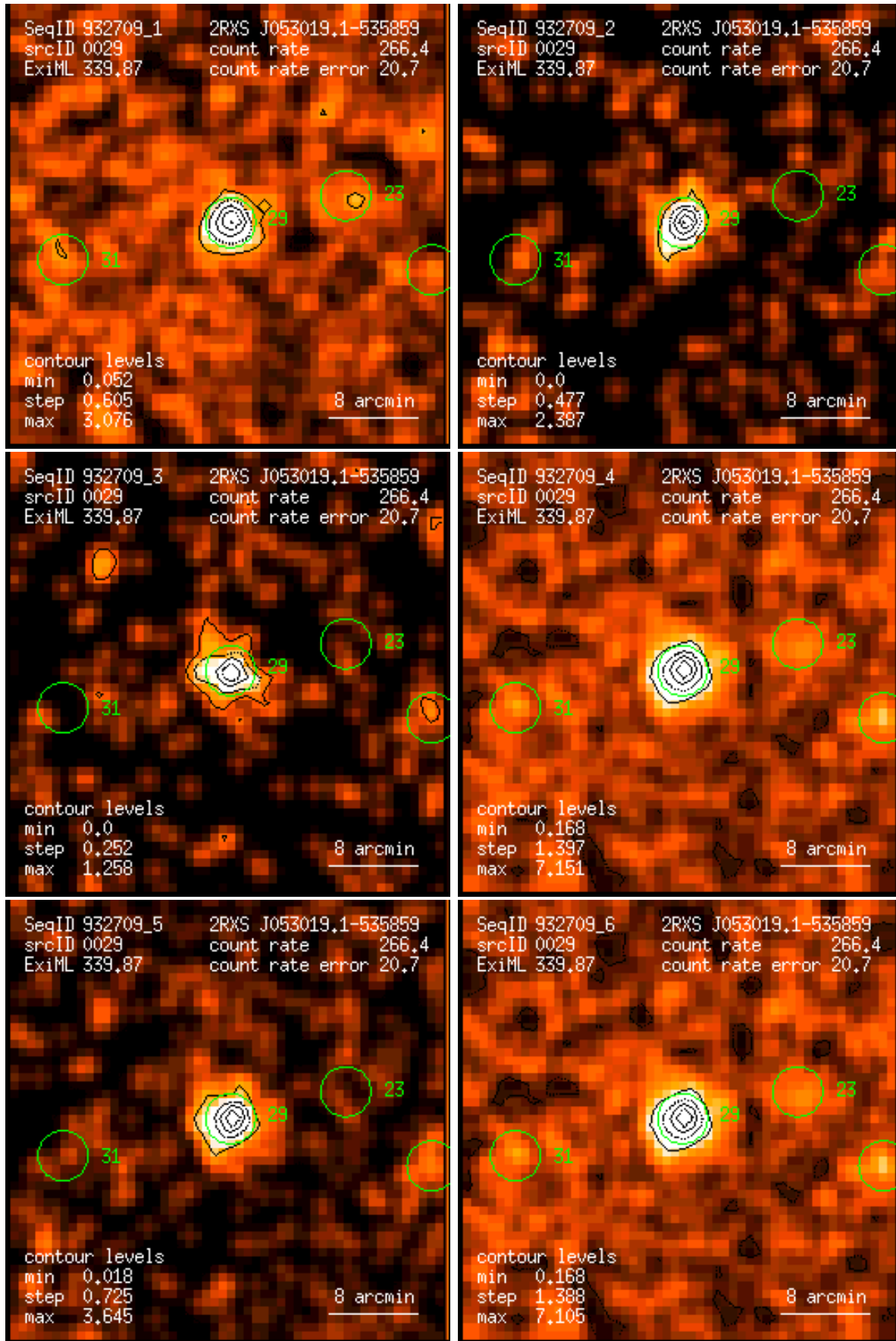
Figure 29: RASS 932709: detection 0029: band rate images, Gaussian filter: (1) PSPC channels 11 – 41, (2) 52 – 90, (3) 91 – 201, (4) 11 – 235, (5) 52 – 201, (6) 11 – 201. Broad band rates in counts/ks. Band rate contour levels in counts/ks/arcmin 2 .
