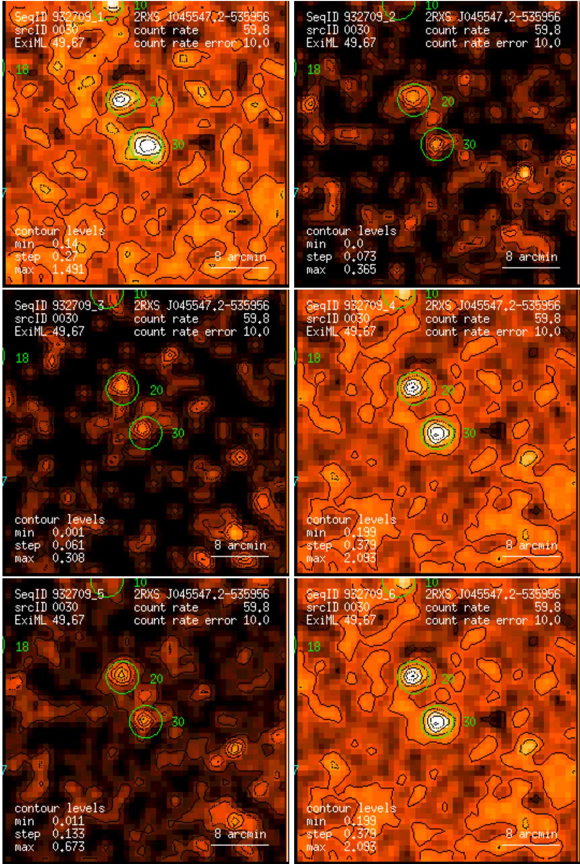
Figure 30: RASS 932709: detection 0030: band rate images, Gaussian filter: (1) PSPC channels 11 – 41, (2) 52 – 90, (3) 91 – 201, (4) 11 – 235, (5) 52 – 201, (6) 11 – 201. Broad band rates in counts/ks. Band rate contour levels in counts/ks/arcmin 2 .
