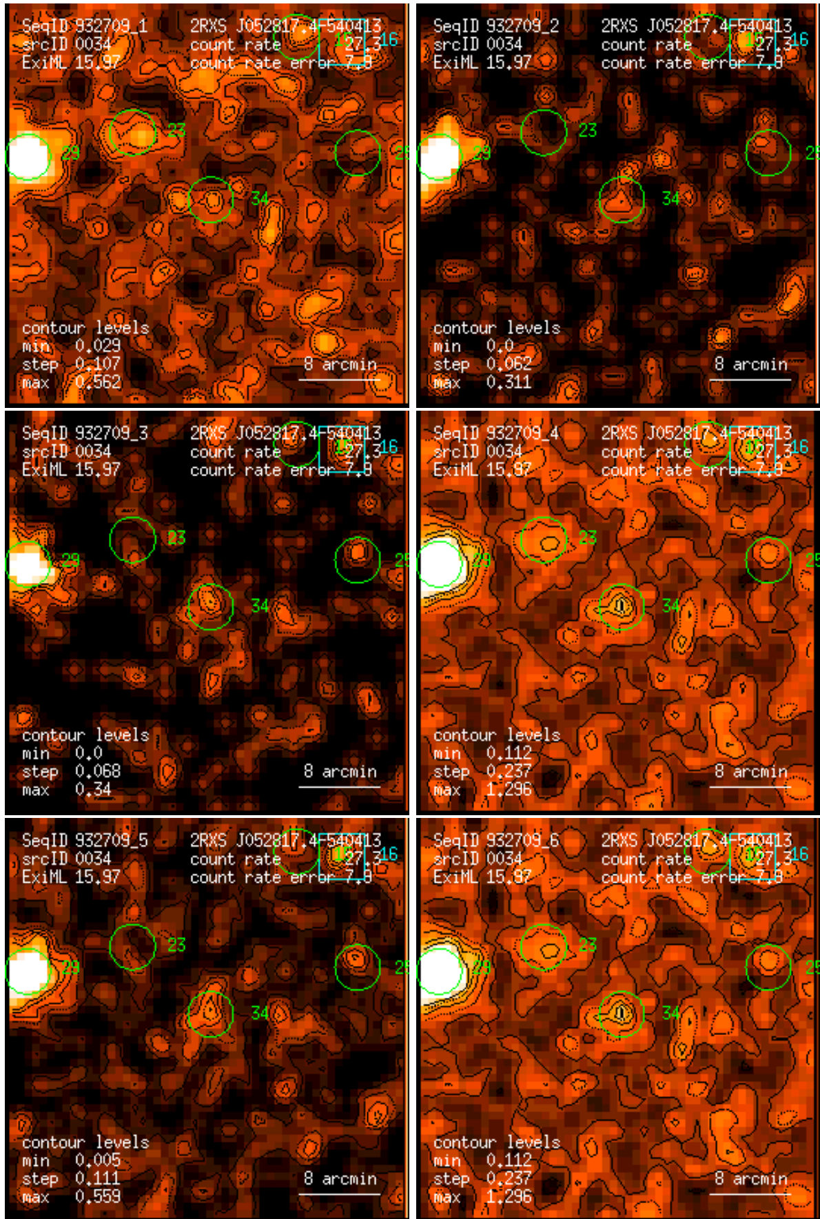
Figure 34: RASS 932709: detection 0034: band rate images, Gaussian filter: (1) PSPC channels 11 – 41, (2) 52 – 90, (3) 91 – 201, (4) 11 – 235, (5) 52 – 201, (6) 11 – 201. Broad band rates in counts/ks. Band rate contour levels in counts/ks/arcmin 2 .
