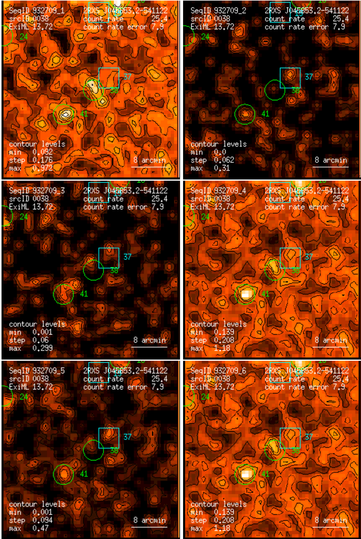
Figure 38: RASS 932709: detection 0038: band rate images, Gaussian filter: (1) PSPC channels 11 – 41, (2) 52 – 90, (3) 91 – 201, (4) 11 – 235, (5) 52 – 201, (6) 11 – 201. Broad band rates in counts/ks. Band rate contour levels in counts/ks/arcmin 2 .
