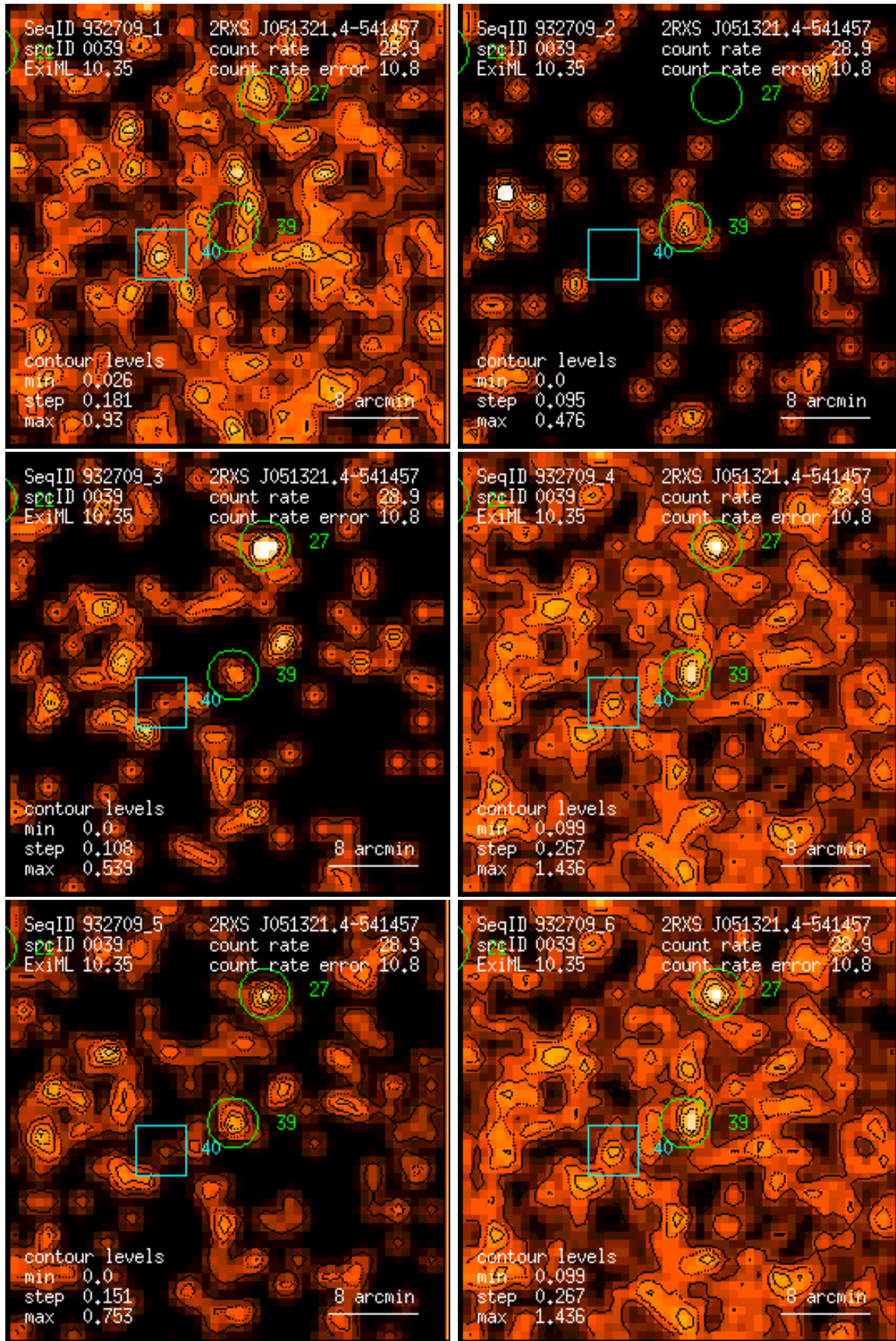
Figure 39: RASS 932709: detection 0039: band rate images, Gaussian filter: (1) PSPC channels 11 – 41, (2) 52 – 90, (3) 91 – 201, (4) 11 – 235, (5) 52 – 201, (6) 11 – 201. Broad band rates in counts/ks. Band rate contour levels in counts/ks/arcmin 2 .
