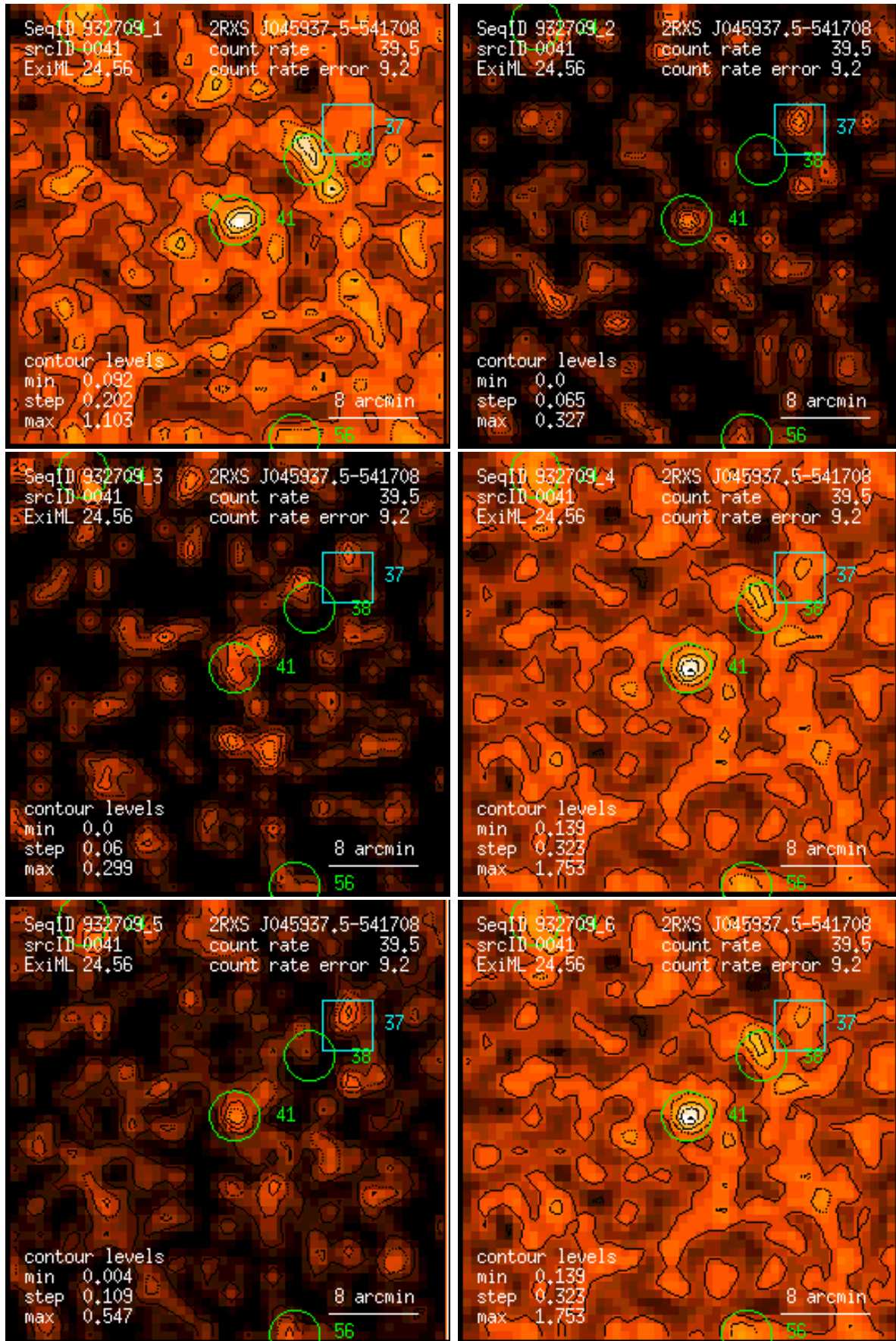
Figure 41: RASS 932709: detection 0041: band rate images, Gaussian filter: (1) PSPC channels 11 – 41, (2) 52 – 90, (3) 91 – 201, (4) 11 – 235, (5) 52 – 201, (6) 11 – 201. Broad band rates in counts/ks. Band rate contour levels in counts/ks/arcmin 2 .
