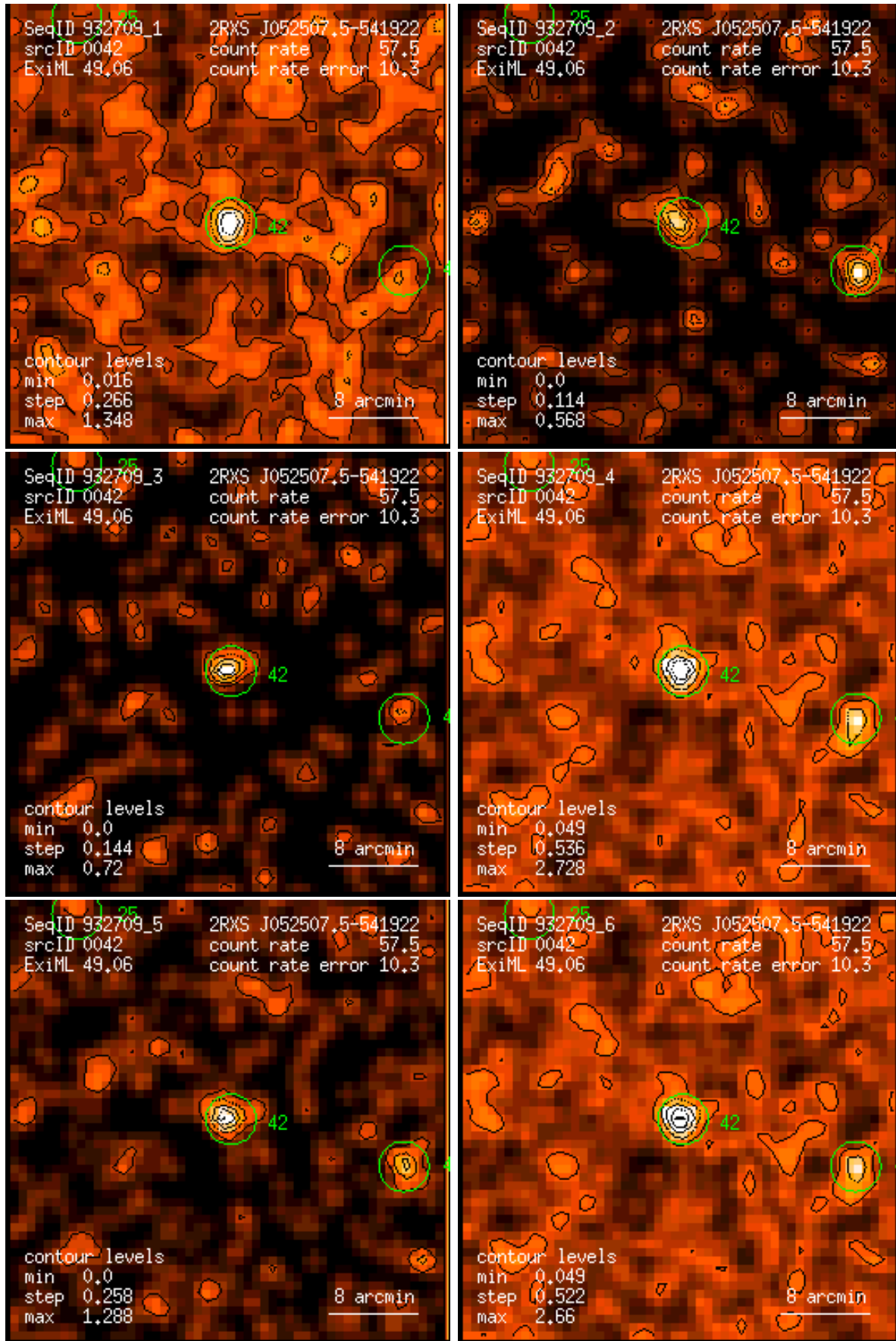
Figure 42: RASS 932709: detection 0042: band rate images, Gaussian filter: (1) PSPC channels 11 – 41, (2) 52 – 90, (3) 91 – 201, (4) 11 – 235, (5) 52 – 201, (6) 11 – 201. Broad band rates in counts/ks. Band rate contour levels in counts/ks/arcmin 2 .
