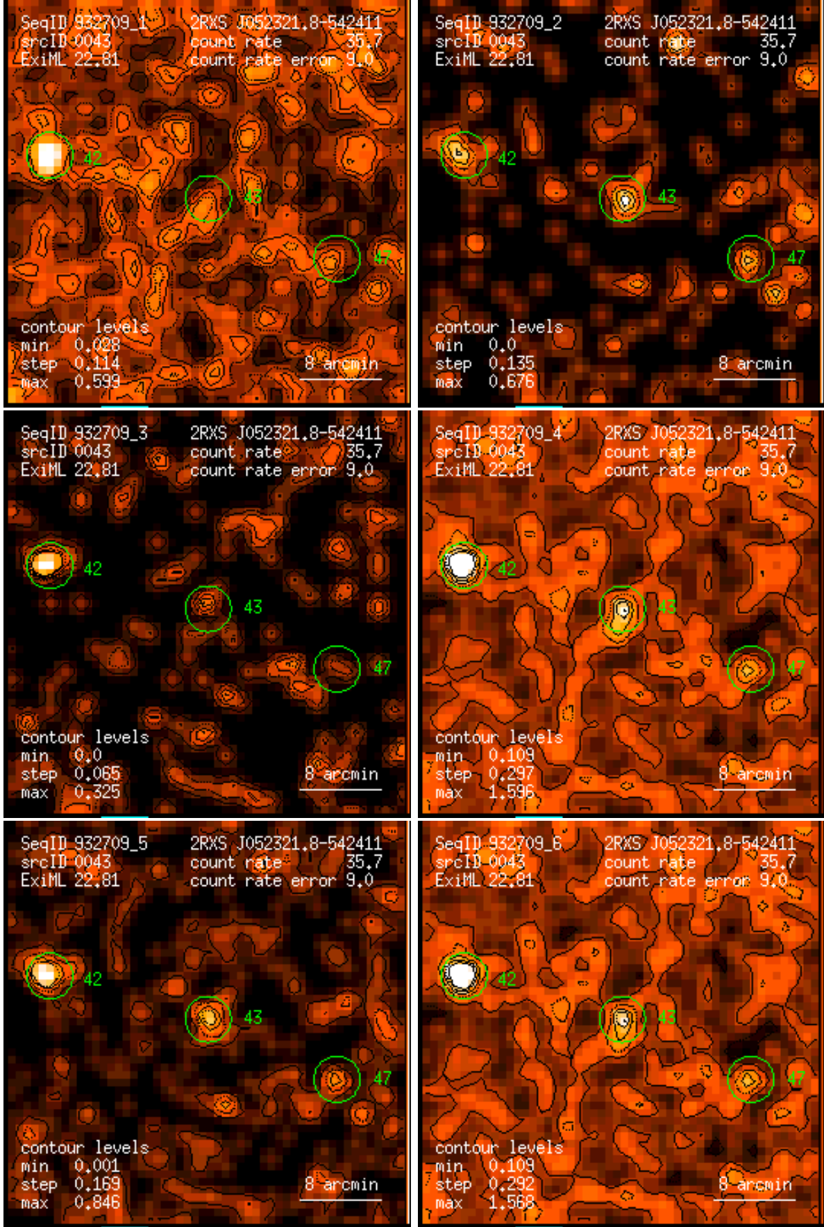
Figure 43: RASS 932709: detection 0043: band rate images, Gaussian filter: (1) PSPC channels 11 – 41, (2) 52 – 90, (3) 91 – 201, (4) 11 – 235, (5) 52 – 201, (6) 11 – 201. Broad band rates in counts/ks. Band rate contour levels in counts/ks/arcmin 2 .
