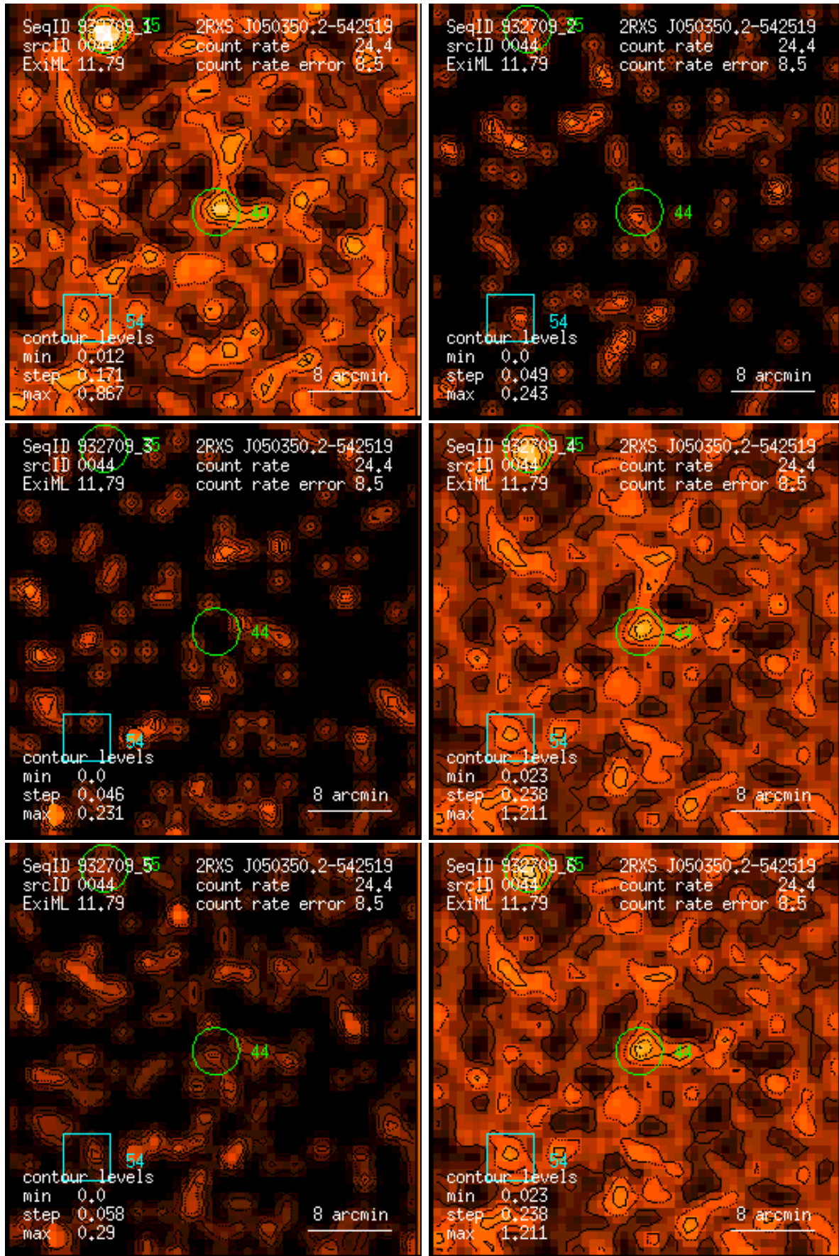
Figure 44: RASS 932709: detection 0044: band rate images, Gaussian filter: (1) PSPC channels 11 – 41, (2) 52 – 90, (3) 91 – 201, (4) 11 – 235, (5) 52 – 201, (6) 11 – 201. Broad band rates in counts/ks. Band rate contour levels in counts/ks/arcmin 2 .
