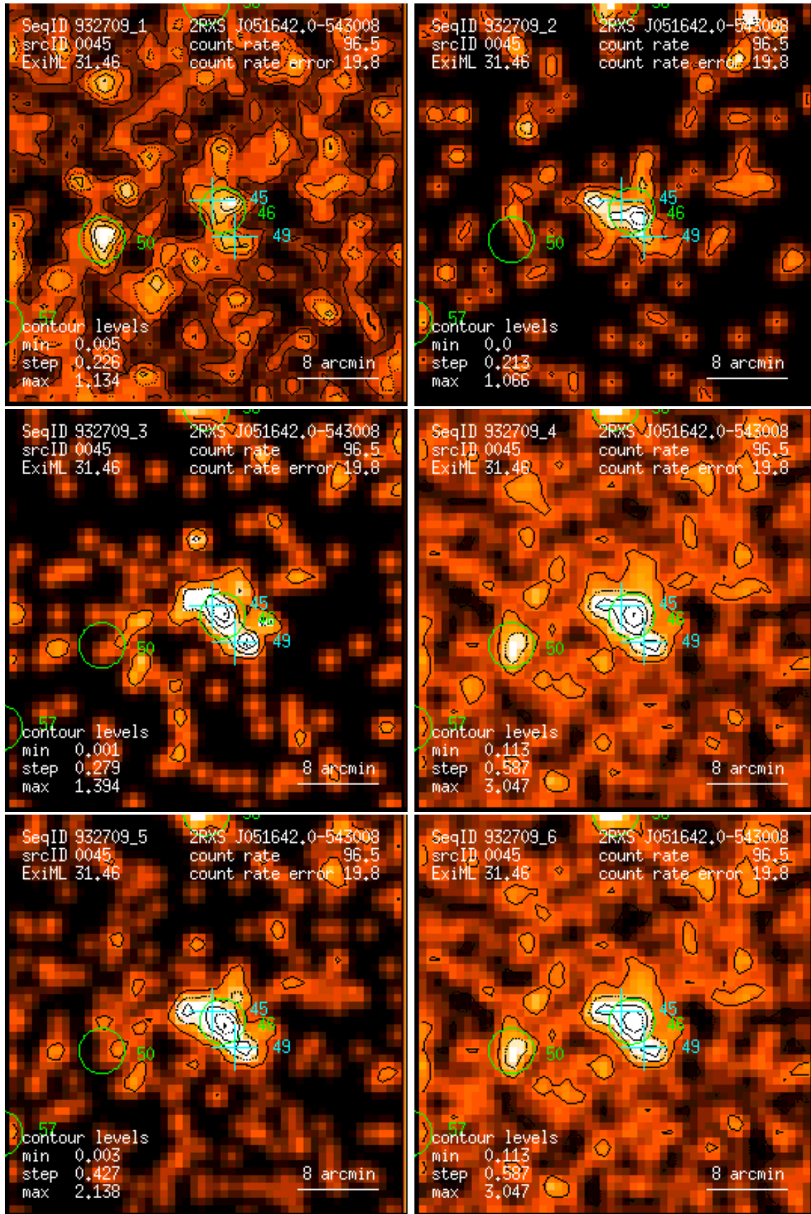
Figure 45: RASS 932709: detection 0045: band rate images, Gaussian filter: (1) PSPC channels 11 – 41, (2) 52 – 90, (3) 91 – 201, (4) 11 – 235, (5) 52 – 201, (6) 11 – 201. Broad band rates in counts/ks. Band rate contour levels in counts/ks/arcmin 2 .
