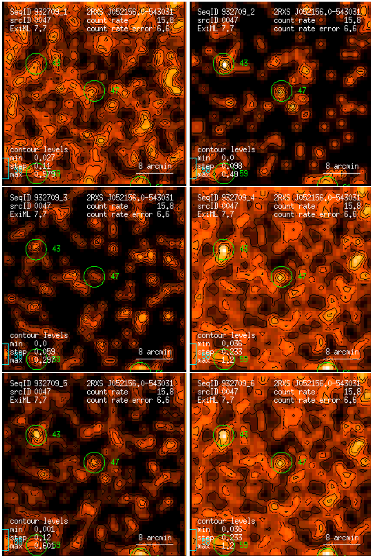
Figure 47: RASS 932709: detection 0047: band rate images, Gaussian filter: (1) PSPC channels 11 – 41, (2) 52 – 90, (3) 91 – 201, (4) 11 – 235, (5) 52 – 201, (6) 11 – 201. Broad band rates in counts/ks. Band rate contour levels in counts/ks/arcmin 2 .
